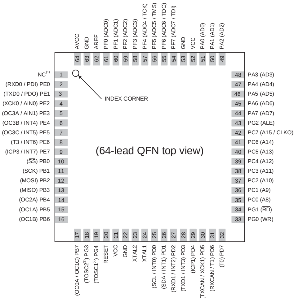
Figure 2-3. Pinout AT90CAN32/64 - QFN
