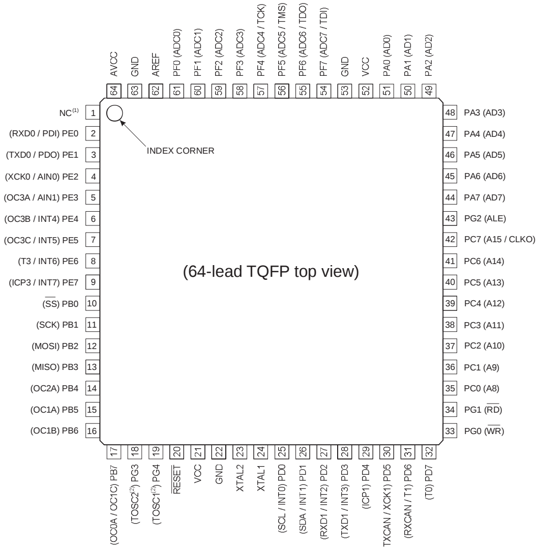
Figure 2-2. Pinout AT90CAN32/64 - TQFP
