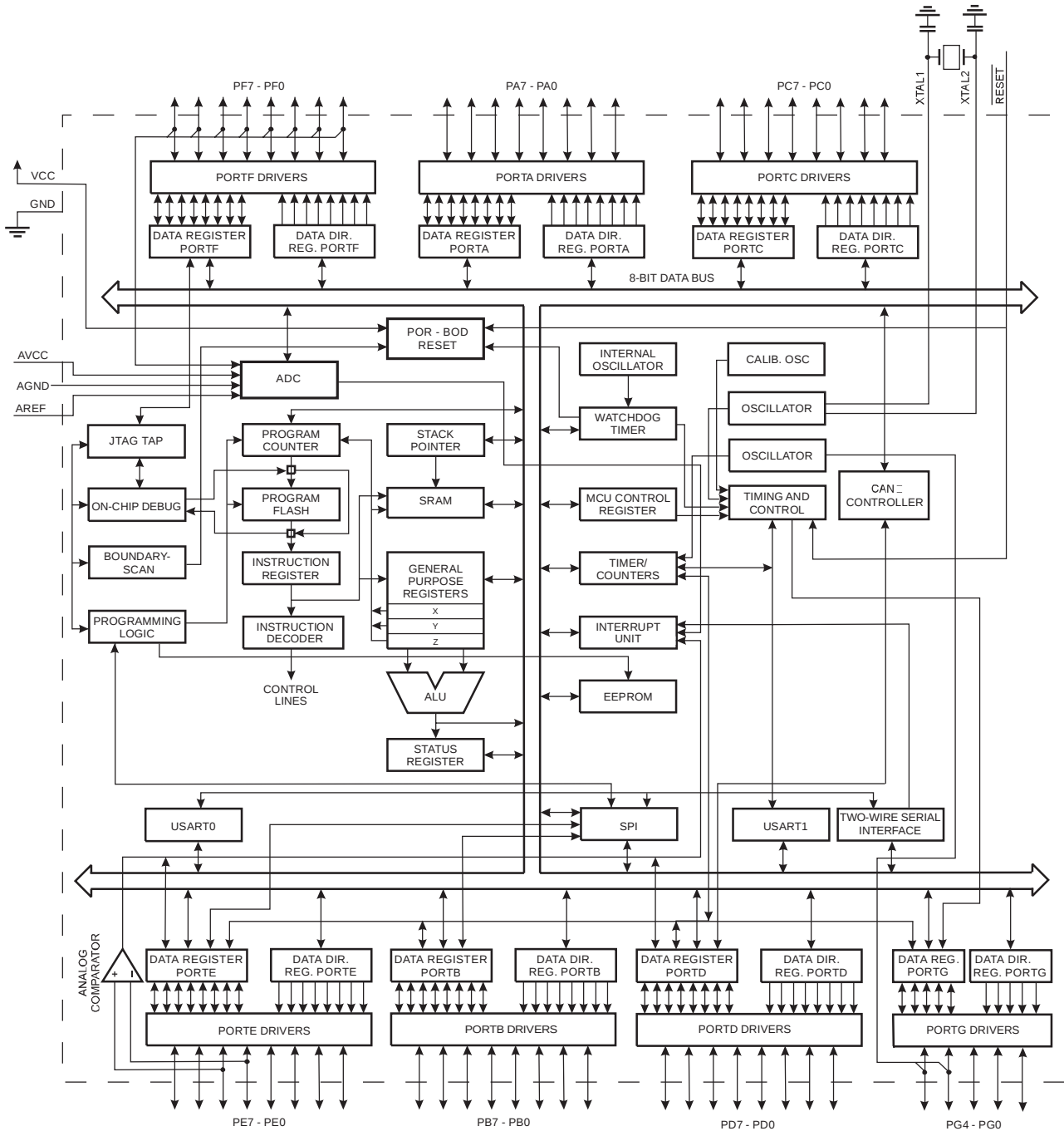
Figure 2-1. Block Diagram
