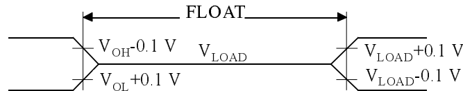
Figure 19-13. Float Waveforms
