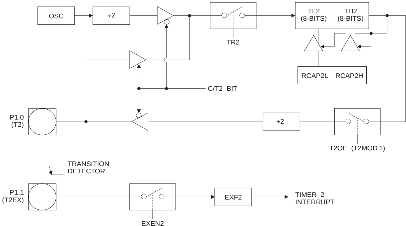
Figure 5. Timer 2 in Clock-Out Mode
