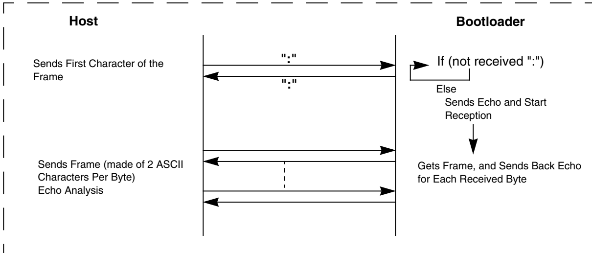
Figure 23-12. Command Flow
