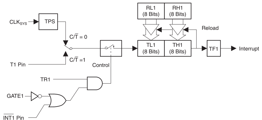
Figure 12-2. Timer/Counter 1 Mode 1: 16-bit Auto-Reload
