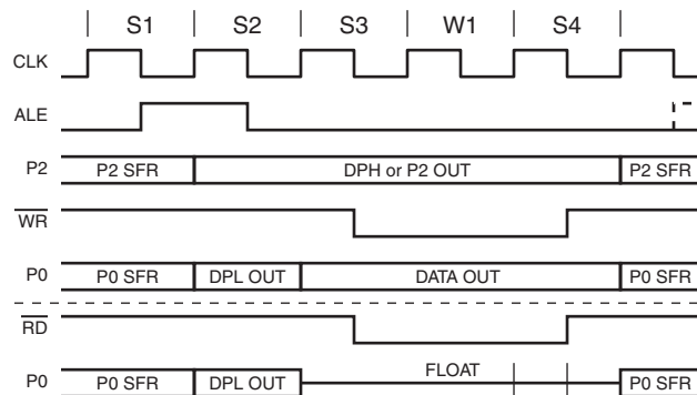
Figure 3-16. MOVX with One Wait State (WS = 01B)
