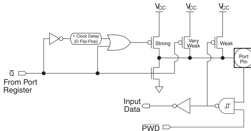
Figure 13-1. Quasi-bidirectional Output
