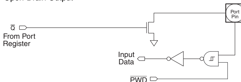
Figure 13-4. Open-Drain Output
