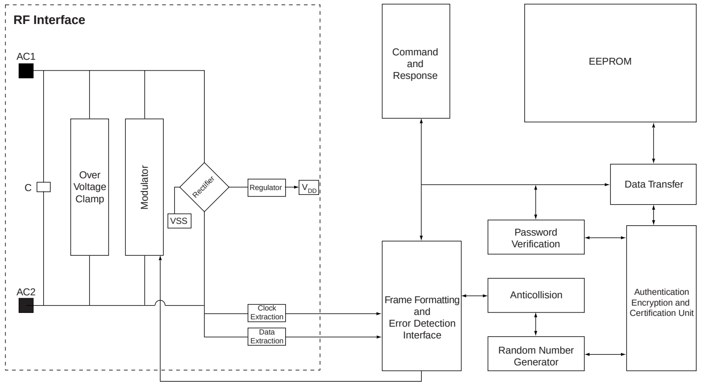
Figure 1. Block Diagram
