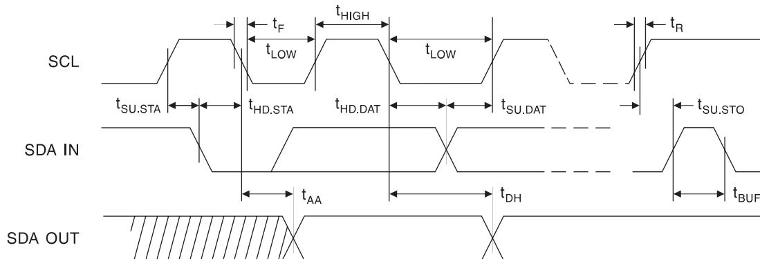
Figure 10-1. Bus Timing:
