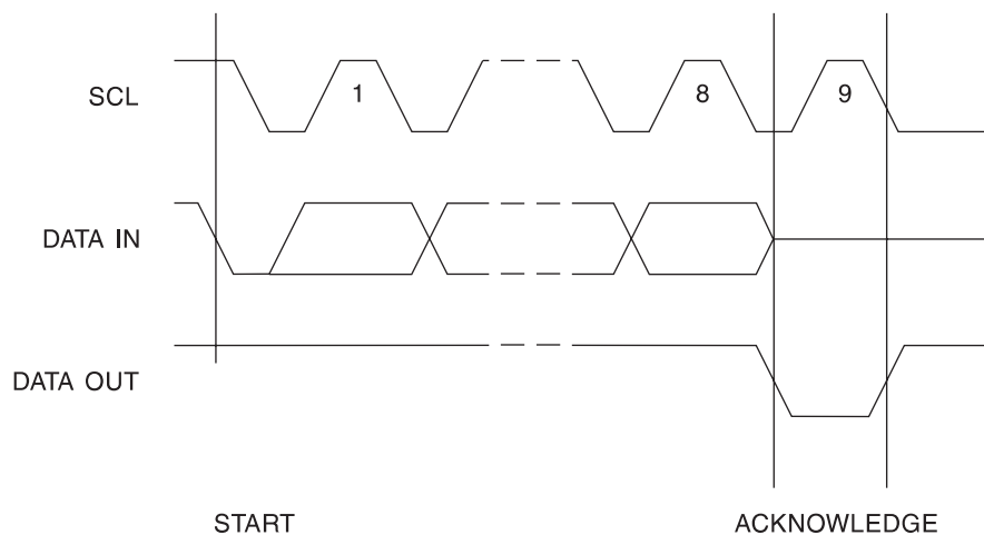
Figure 10-5. Output Acknowledge
