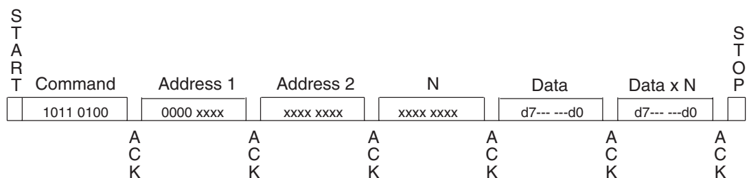
Figure 7-8. System Write
