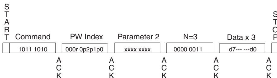
Figure 7-11. Verify Password
