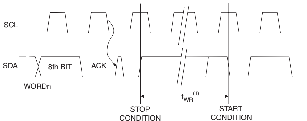
Figure 10-2. Write Cycle Timing:
