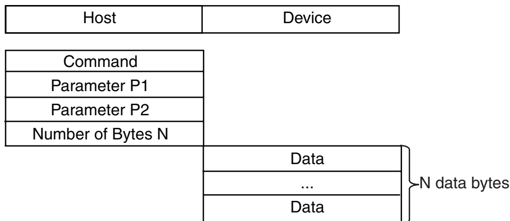
Figure 8-4. System READ Command Functional Description
