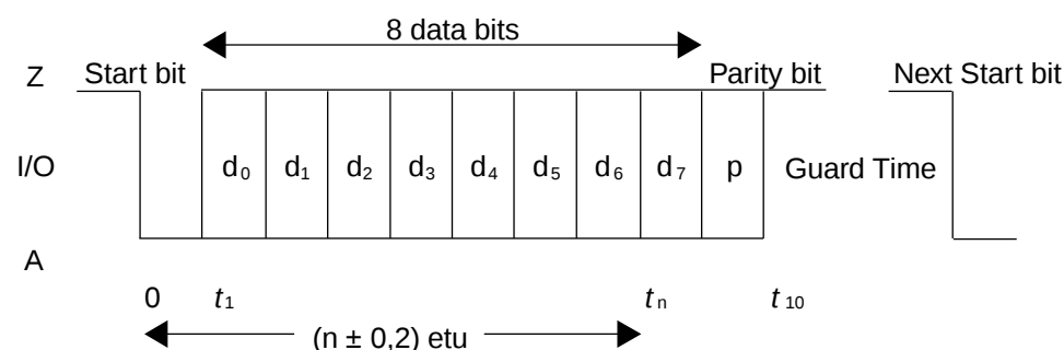
Figure 10-1. Character Format
