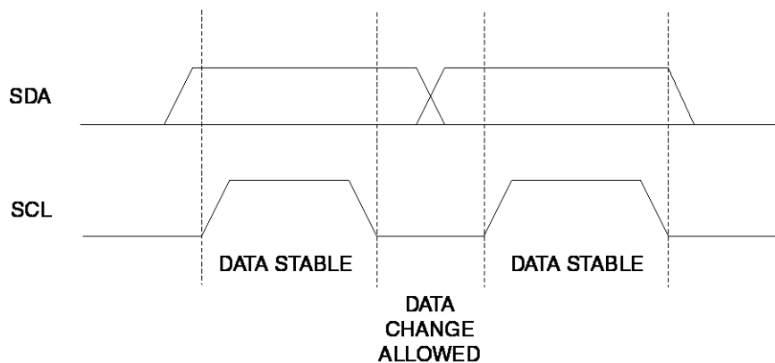
Figure 12-3. Data Validity
