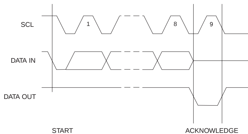
Figure 12-5. Output Acknowledge
