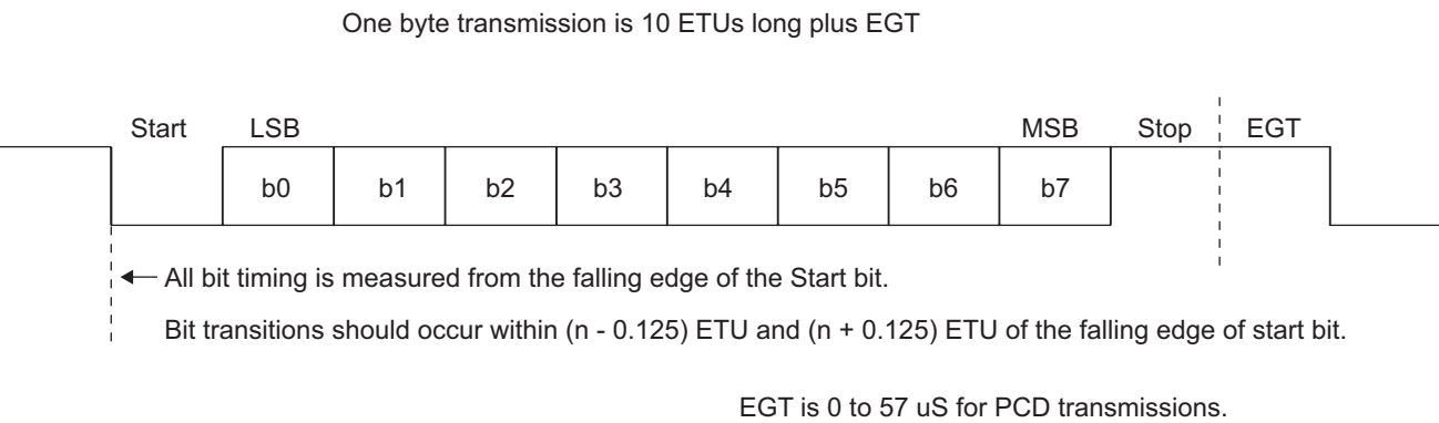
Figure O-1. Byte transmission format requirements for type B communications.
