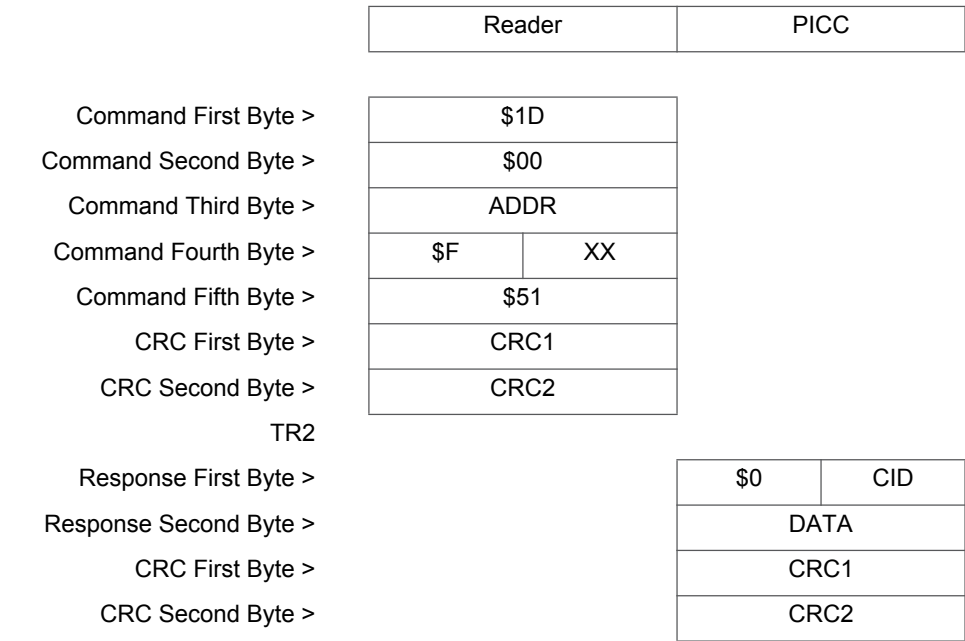
Figure 2-1. Example Command and Response Format
