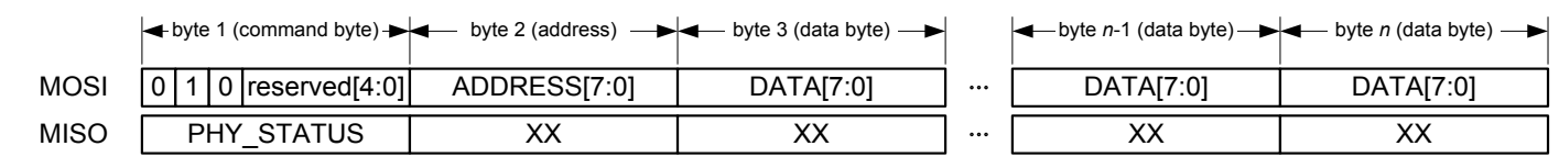
Figure 6-12. Packet Structure – SRAM Write Access.
