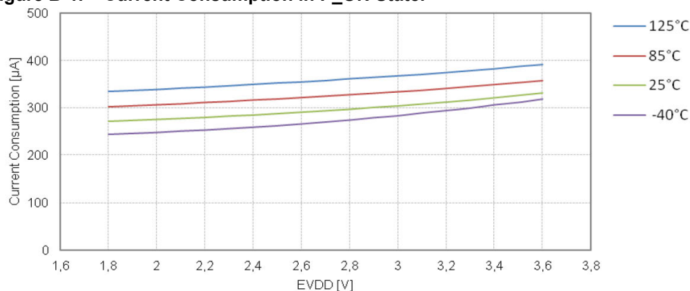
Figure B-1. Current Consumption in P_ON State.
