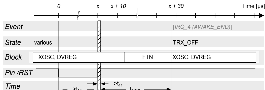
Figure 7-8. Reset Procedure.
