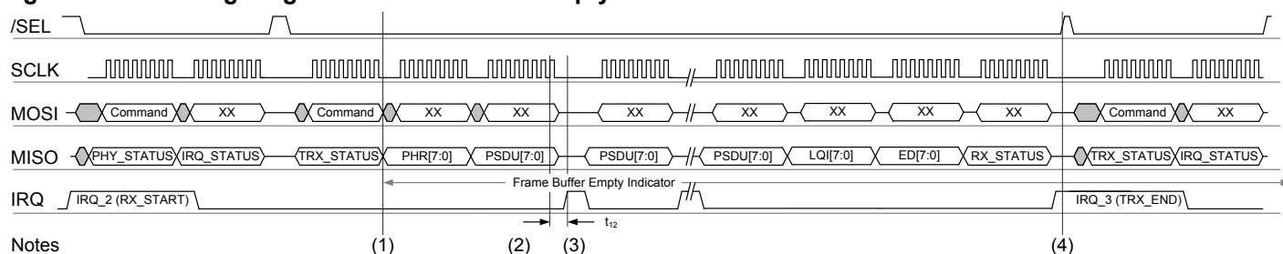
Figure 11-25. Timing Diagram of Frame Buffer Empty Indicator.
