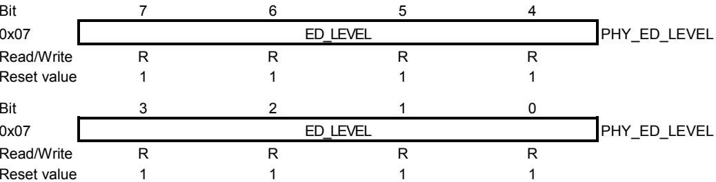
Figure 8-21. Register PHY_ED_LEVEL.
