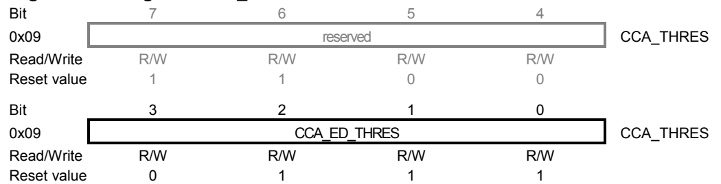
Figure 8-24. Register CCA_THRES.
