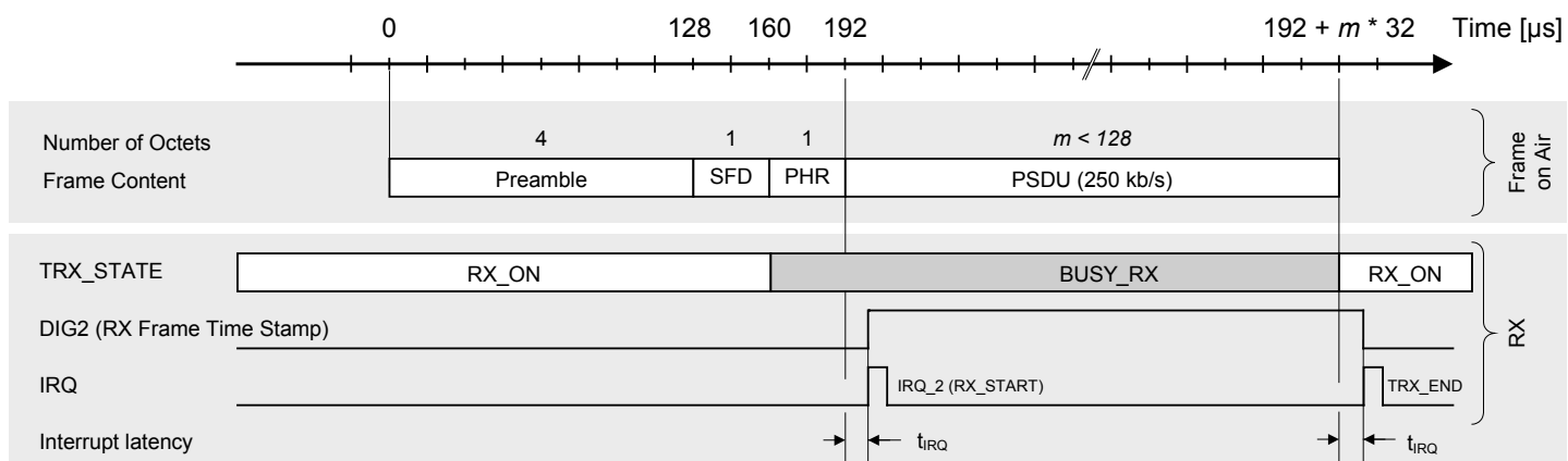
Figure 11-22. Timing of RX_START and DIG2 for RX Frame Time Stamping.
