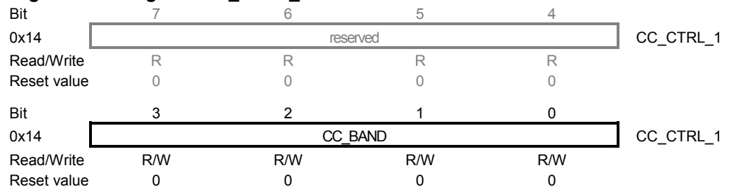
Figure 9-20. Register CC_CTRL_1.
