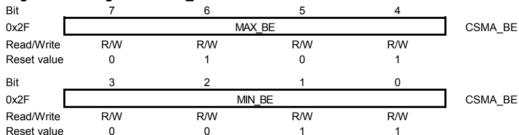
Figure 7-25. Register CSMA_BE.
