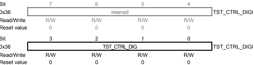
Figure A-1. Register TST_CTRL_DIGI.
