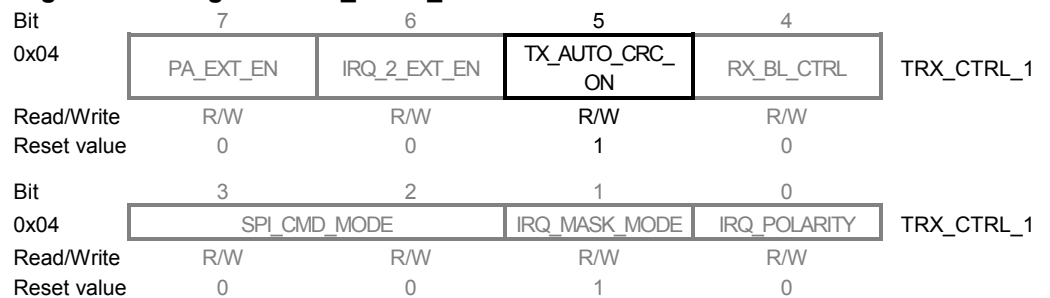
Figure 7-19. Register TRX_CTRL_1.
