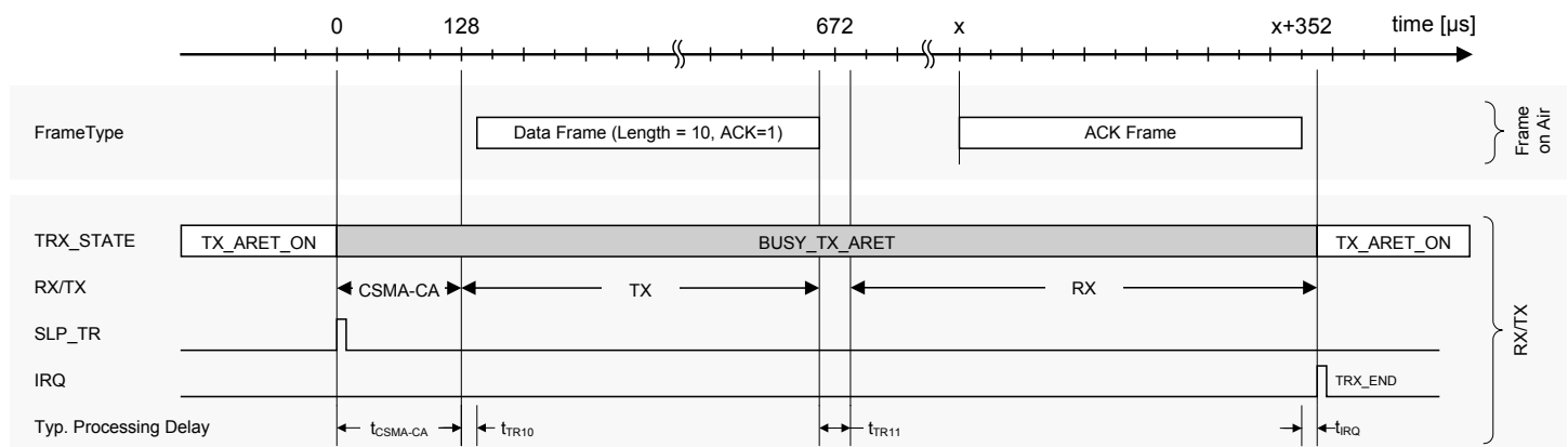
Figure 7-16. Timing Example of a TX_ARET Transaction.
