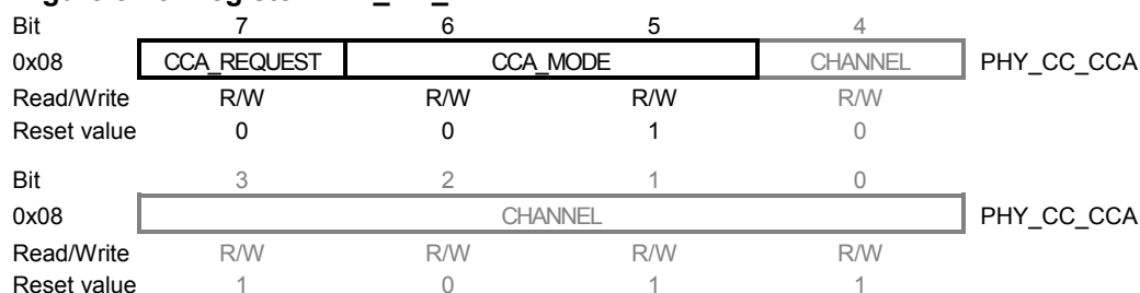
Figure 8-23. Register PHY_CC_CCA.
