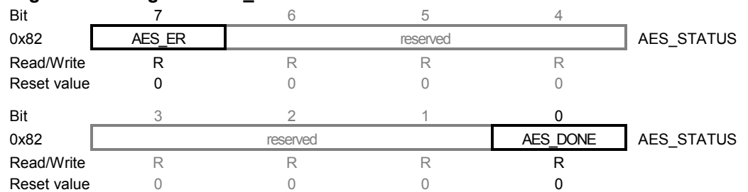
Figure 11-6. Register AES_STATUS.
