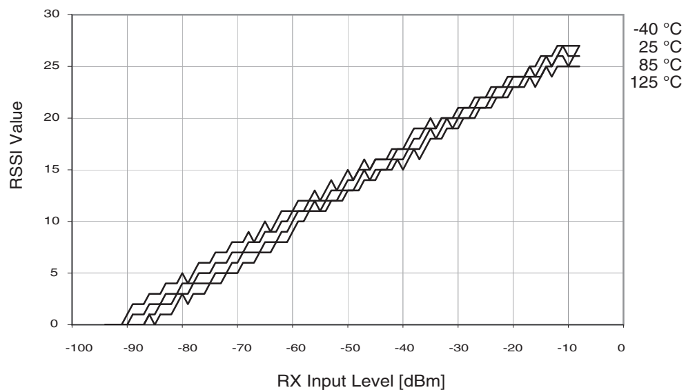
Figure 21-16. RSSI
