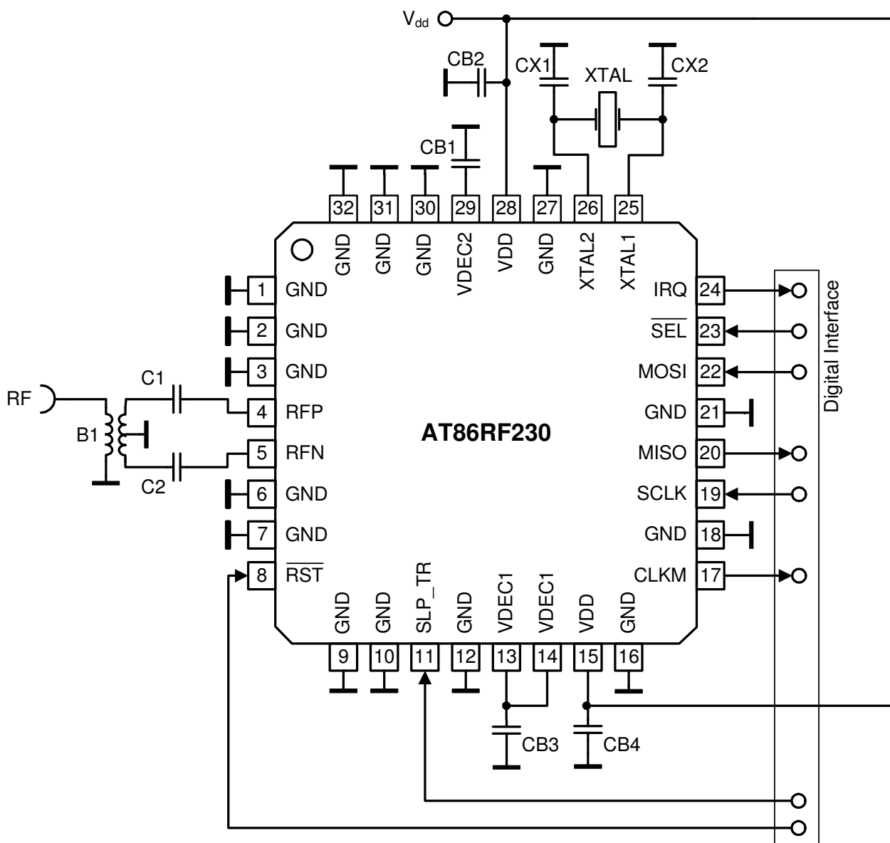
Figure 9-1. Application Schematic
