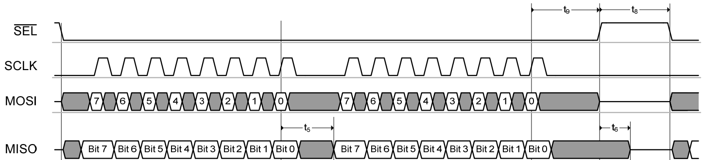
Figure 6-2. SPI Timing, Global Map and Definition of Timing Parameters t_5 , t_6 , t_8 and t_9
