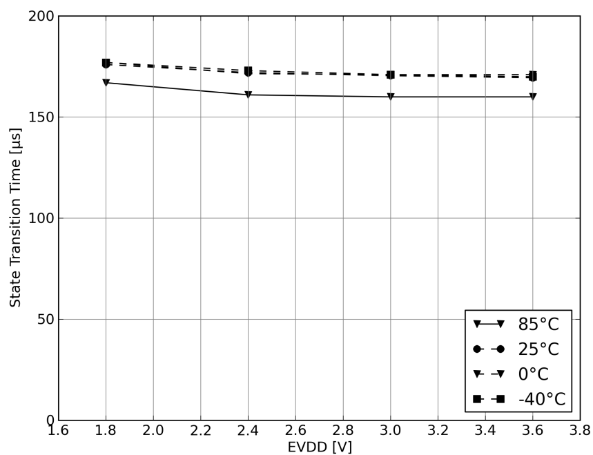
Figure 13-14. Transition Time from TRX_OFF to PLL_ON.
