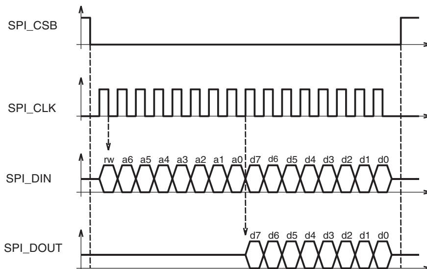
Figure 8-1. SPI Architecture
