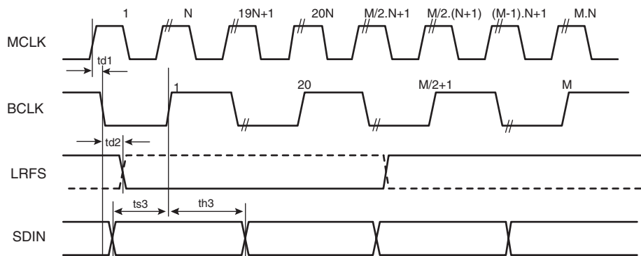
Figure 7-7. Data Interface Timing Diagram
