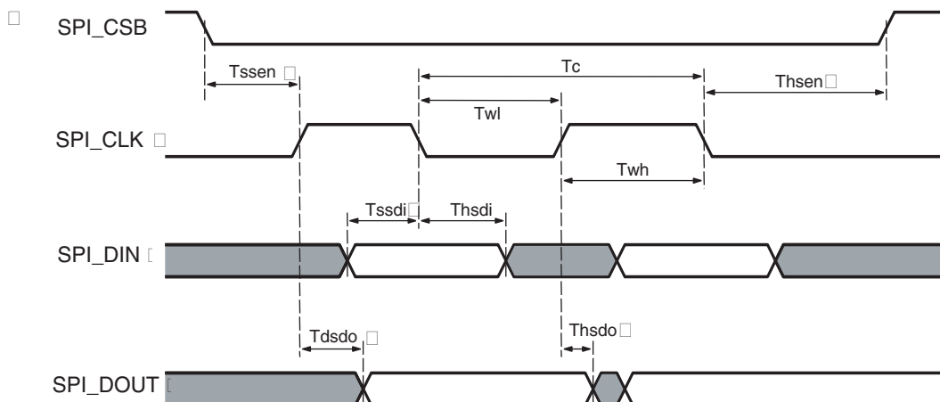
Figure 8-2. SPI Timing
