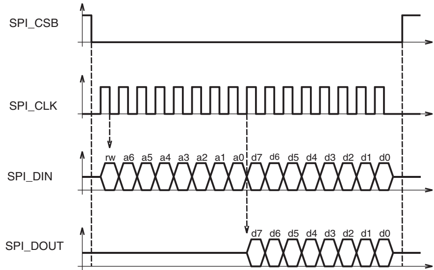
Figure 8-1. SPI Architecture
