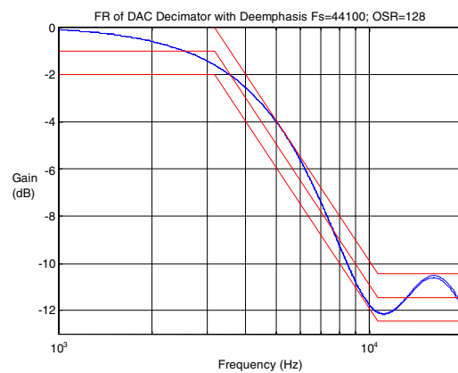
Figure 7-3. De-emphasis Filter
