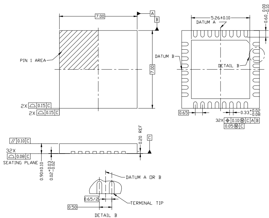
Figure 12-1. Package Outline
