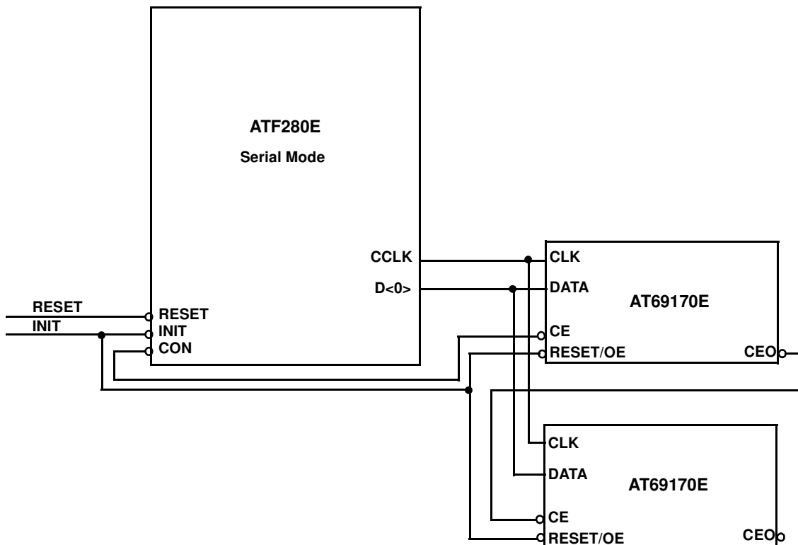
Figure 8-2. AT69170E Cascade
