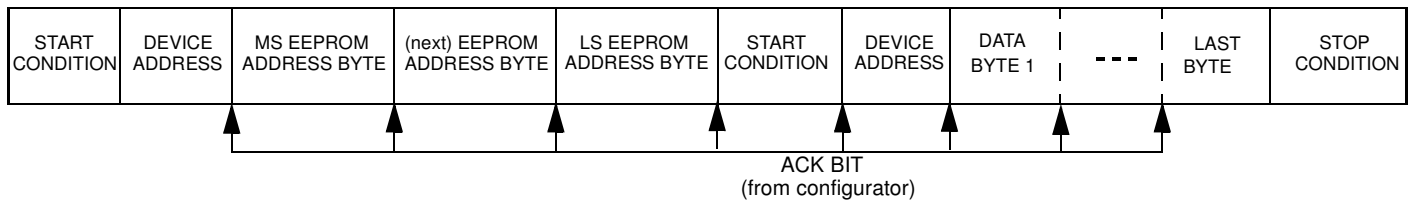
Figure 7-7. Random Read frame
