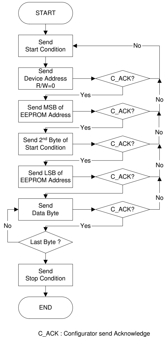
Figure 7-3. Page Programming Summary - TWI Write
