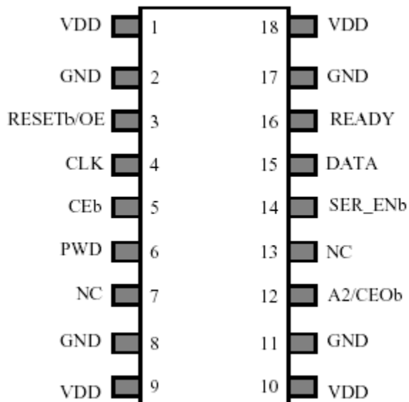
Figure 3-1. AT69170E pin assignment in FP18 package
