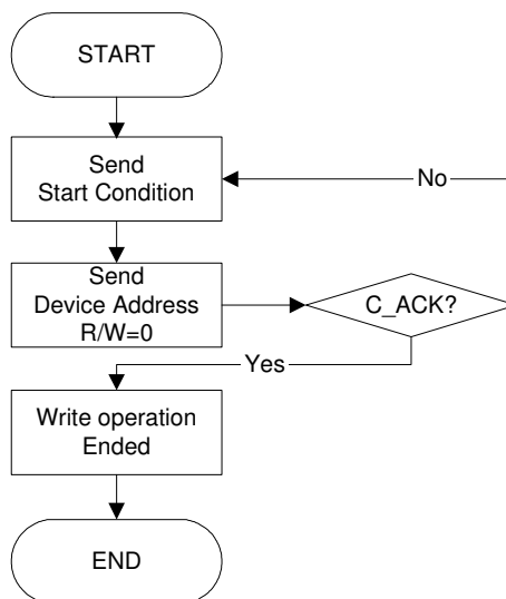
Figure 7-4. Write Polling Summary - TWI Polling
