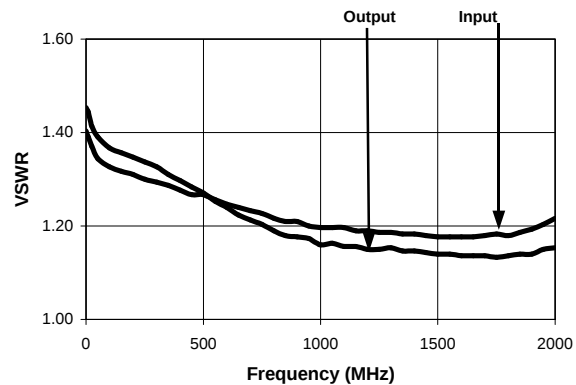
VSWR, 0.5 dB Bit
