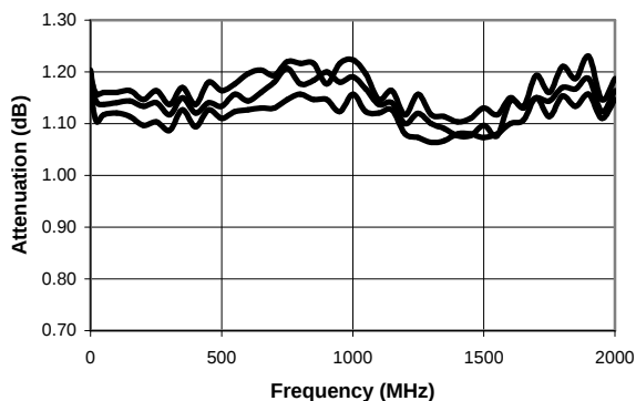
1 dB Bit vs. Temperature
