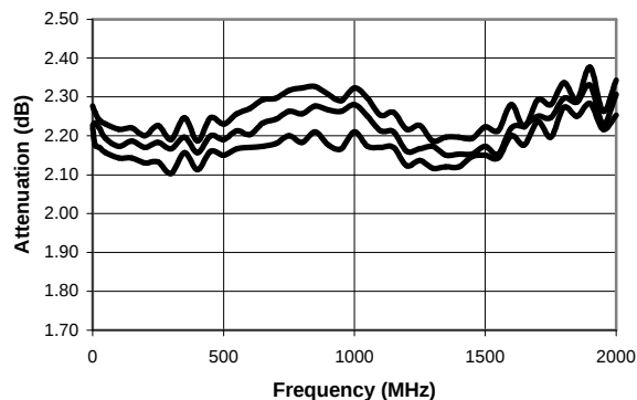
2 dB Bit vs. Temperature
