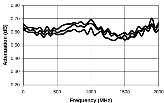
0.5 dB Bit vs. Temperature
