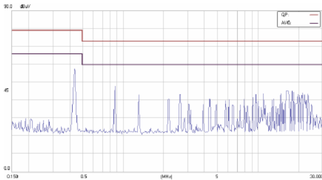
Class A Test Conducted for AT45S3.3-7.5
