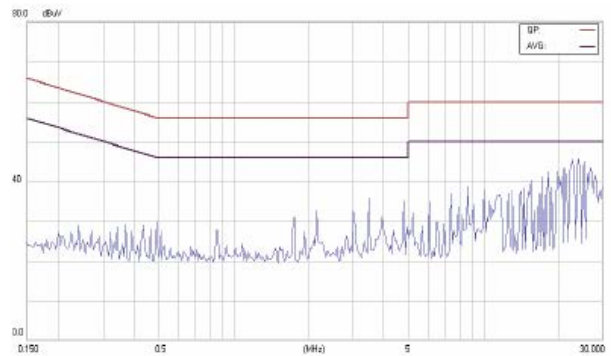
Class B Conducted Test for AT22D15-1
