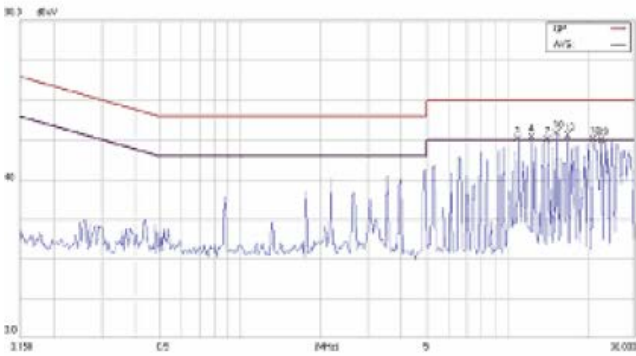
Class B Conducted Test for AT22S12-2.5
