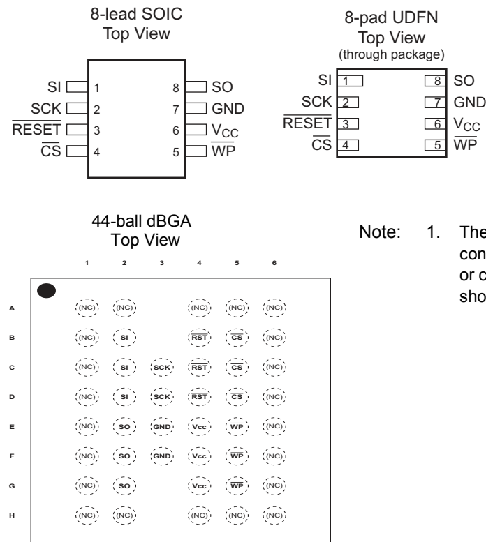
Figure 1-1. Pinouts
