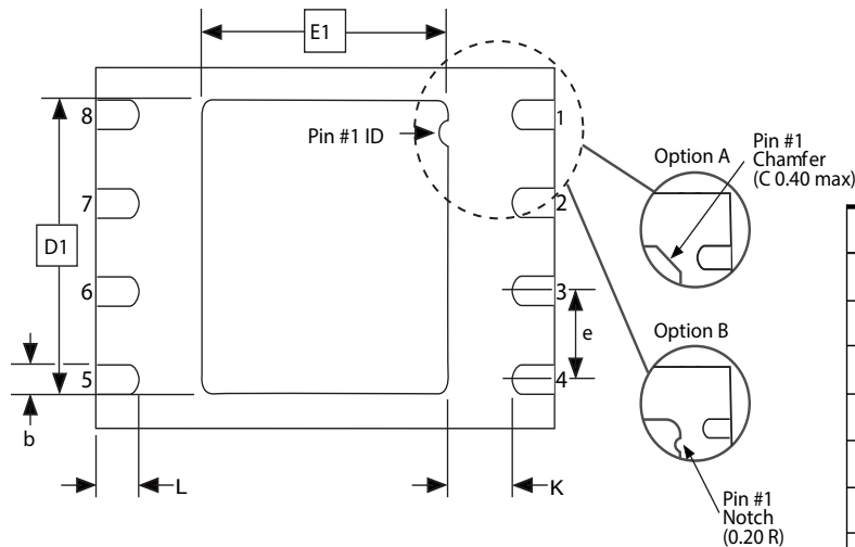
Bottom View
