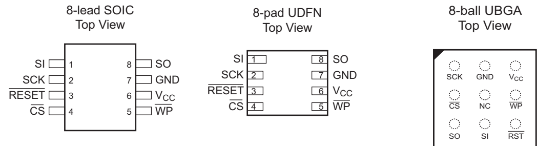
Figure 1-1. Pinouts
