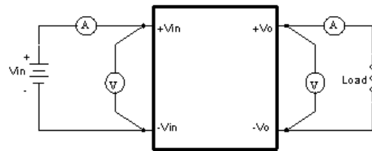
AT Series Test Setup
