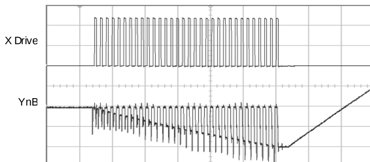
Figure 3-3. VCs – Correct
