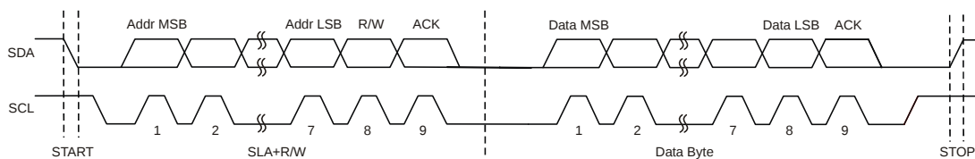
Figure 4-6. Packet Transmission
