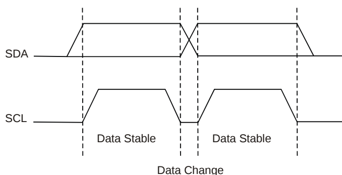
Figure 4-2. Data Transfer
