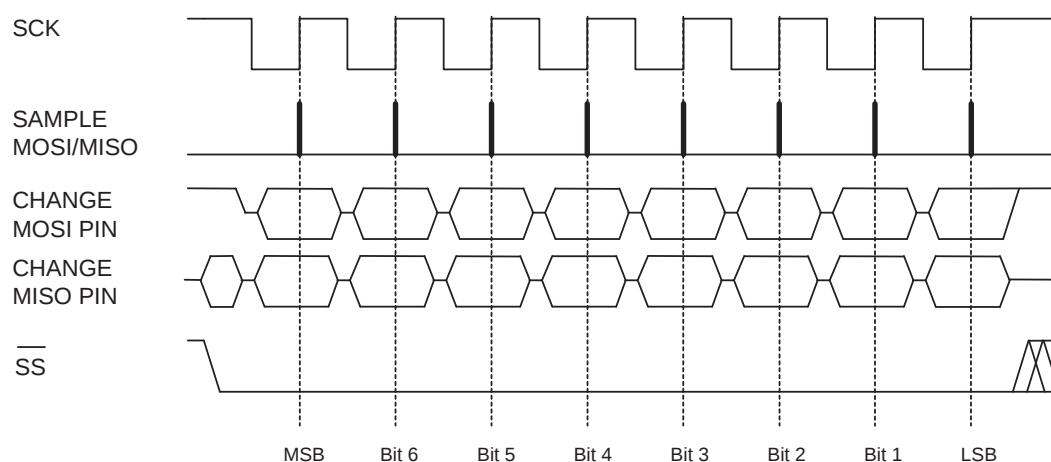
Figure 5-1. SPI Signals
