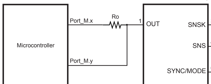
Figure 3-7. Using a Microcontroller to Obtain HeartBeat Pulses in Either Output State (SOT23-6)
