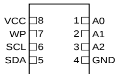
(MLP 2x3) Bottom View
