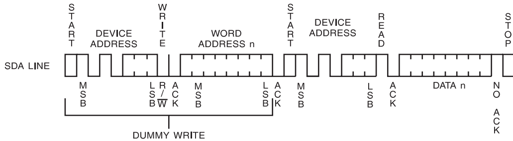
Figure 14. Random Read
