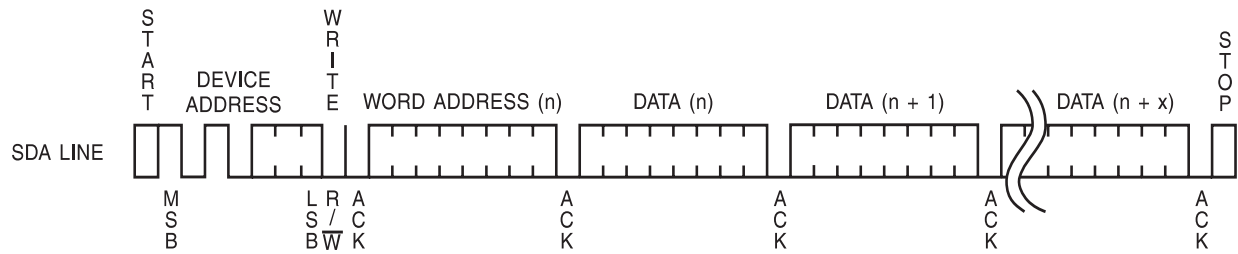
Figure 12. Page Write
