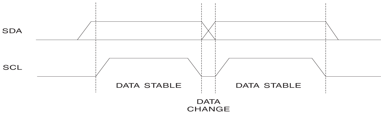
Figure 4. Data Validity
