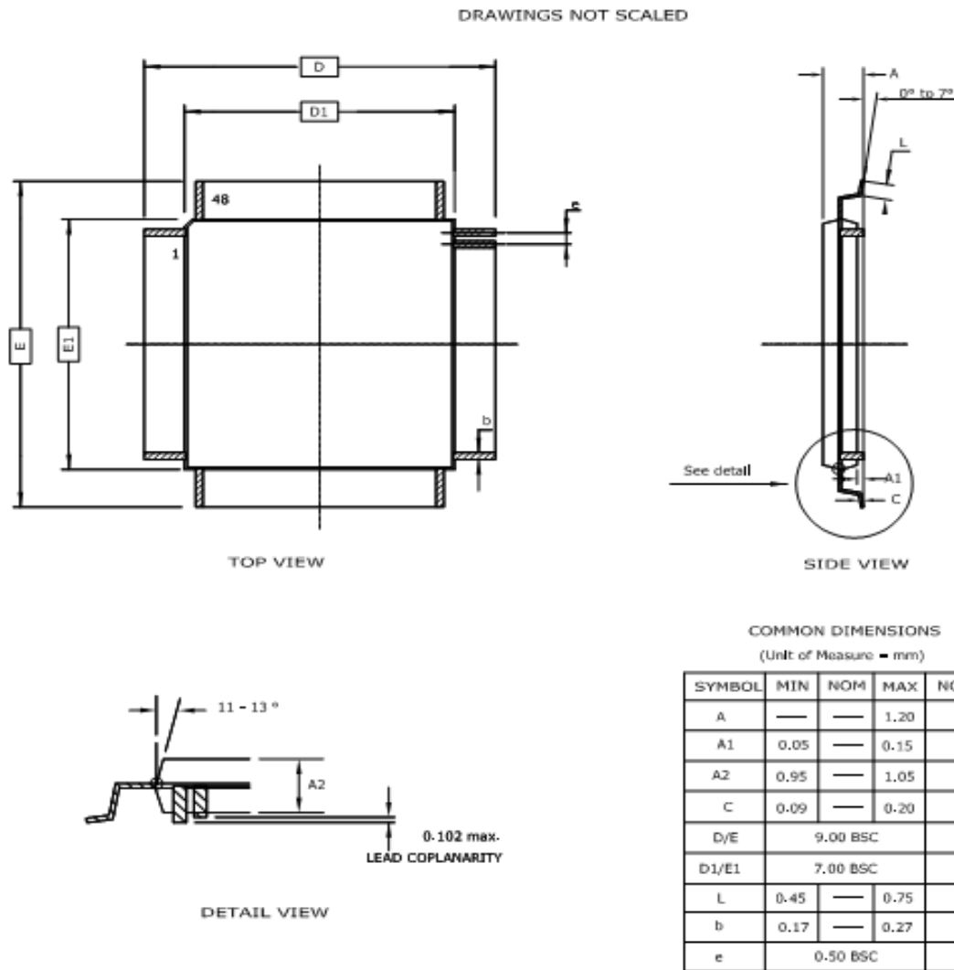
Figure 33-1. TQFP-48 Package Drawing
