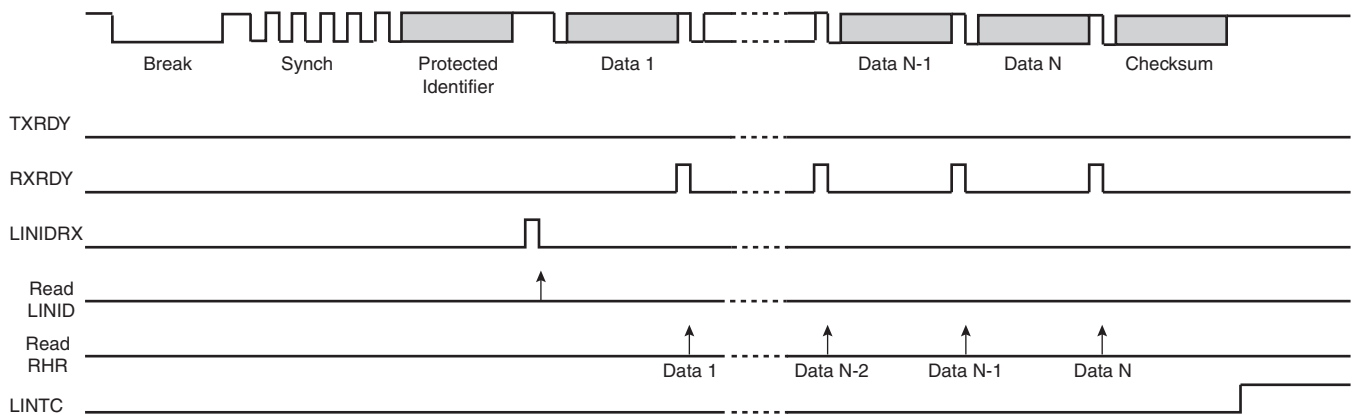
Figure 19-31. Slave Node Configuration, NACT=SUBSCRIBE
