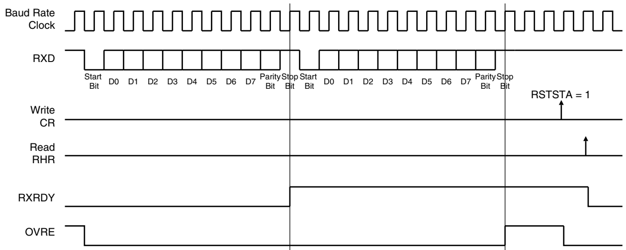
Figure 19-9. Receiver Status
