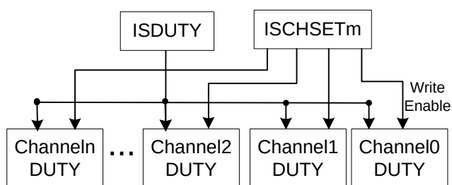
Figure 23-3. Interlinked Single Value PWM Operation Flow
