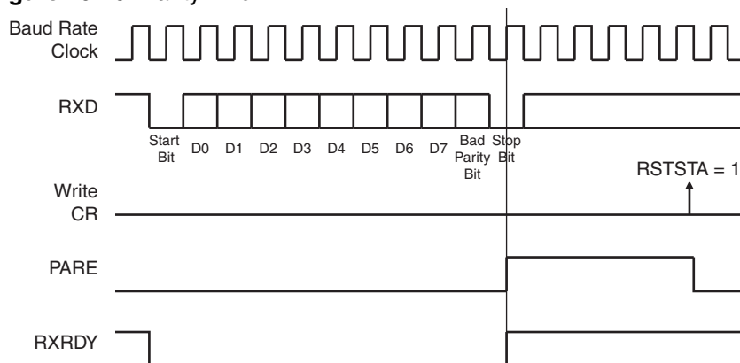
Figure 19-10. Parity Error
