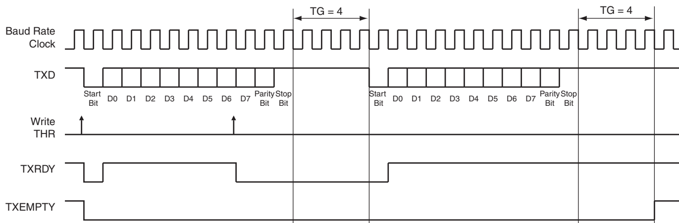
Figure 19-11. Timeguard Operation
