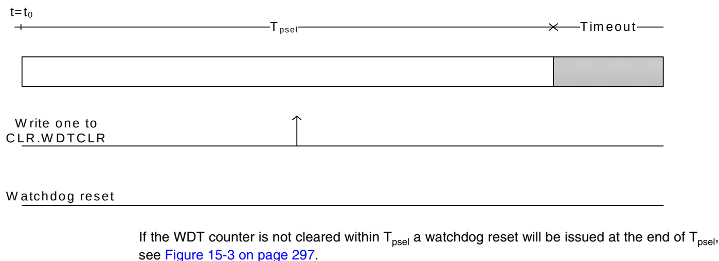
Figure 15-3. Basic Mode WDT Timing Diagram, no clear within T_{psel} .
