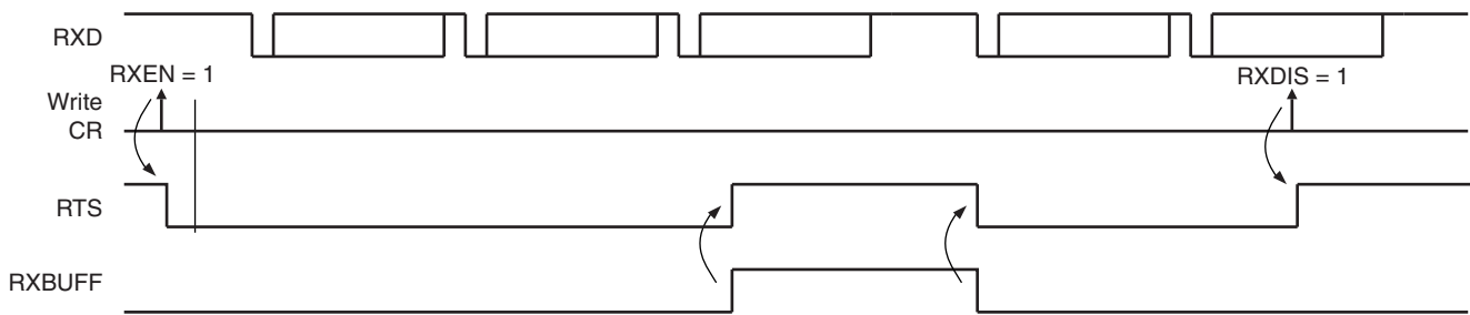
Figure 19-16. Receiver Behavior when Operating with Hardware Handshaking
