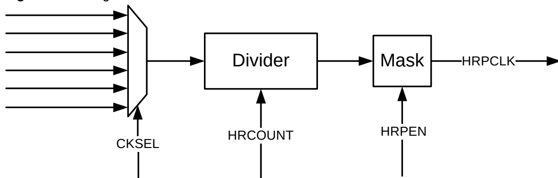
Figure 13-7. High Resolution Prescaler Generation
