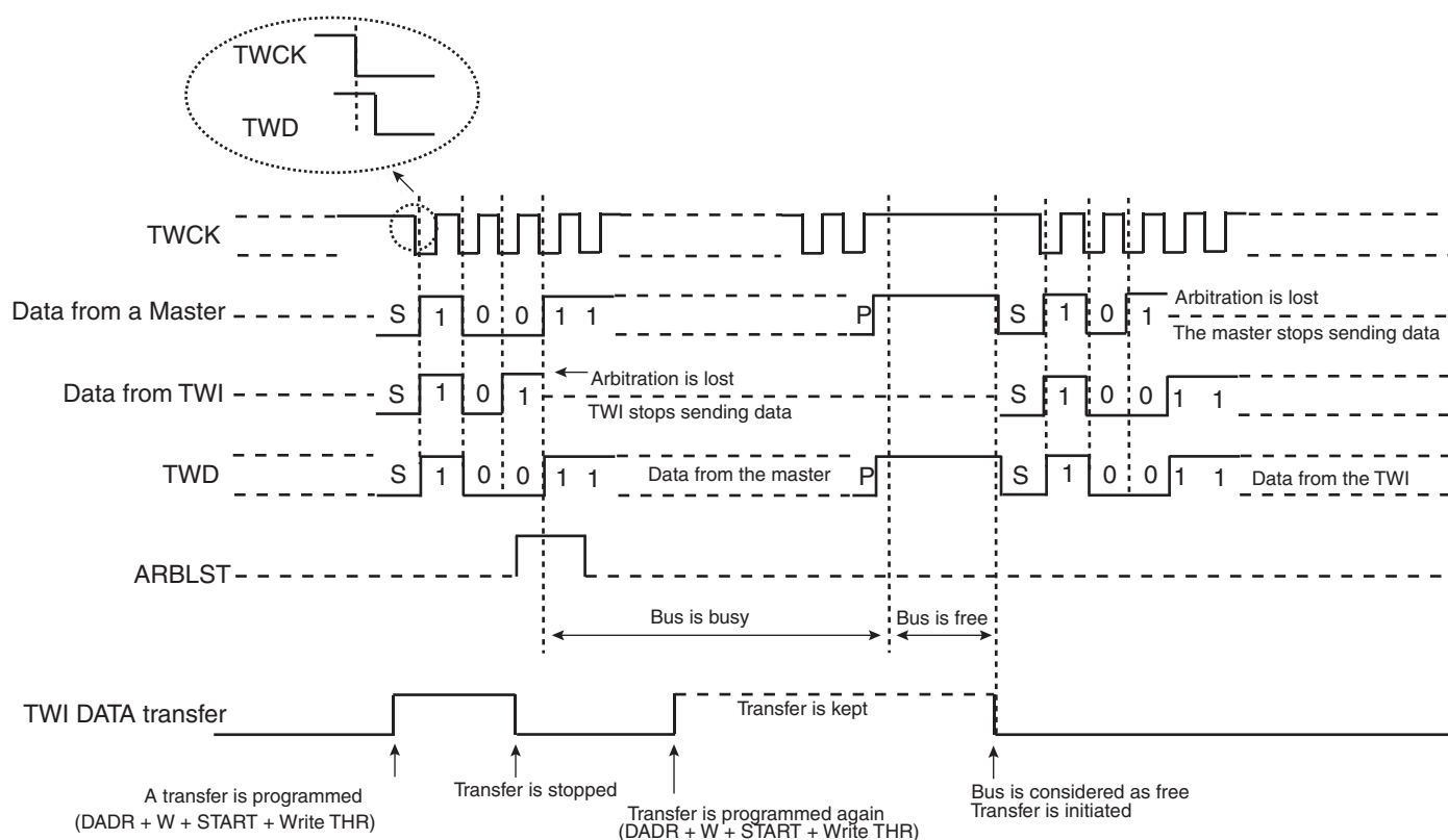
Figure 21-11. Arbitration Cases
