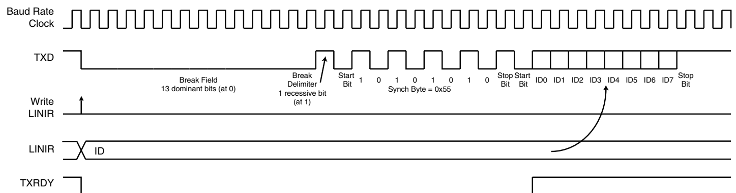
Figure 19-21. Header Transmission
