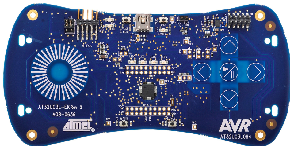
Figure 1-1. AT32UC3L-EK rev2 board
