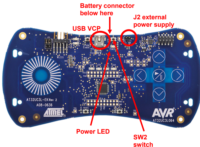
Figure 2-1. Possible power input interfaces on the Atmel AT32UC3L-EK
