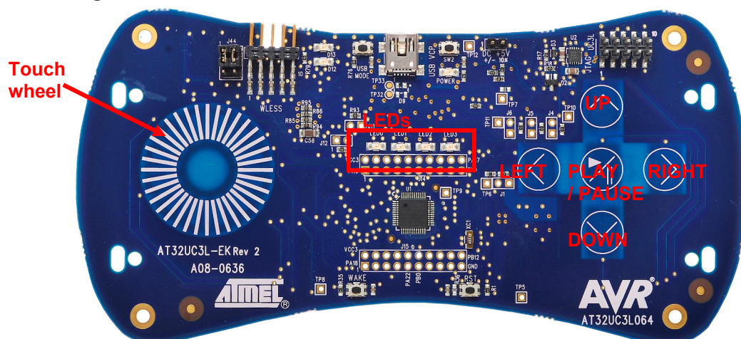
Figure 3-2. Touch sensors and LEDs location
