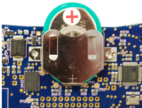
Figure 2-2. Battery and J3 connector (bottom view detail): the side of the battery with the + sign sticker is in contact with the + sign of the J3 connector
