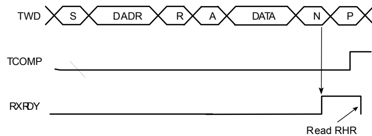
Figure 22-9. Slave Receiver with One Data Byte
