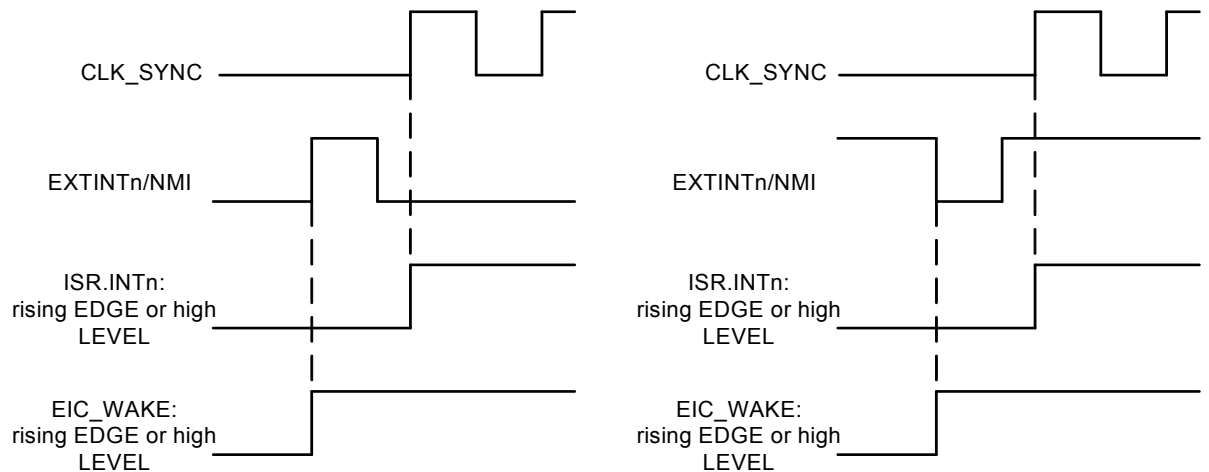
Figure 11-4. Timing Diagram, Asynchronous Interrupts
