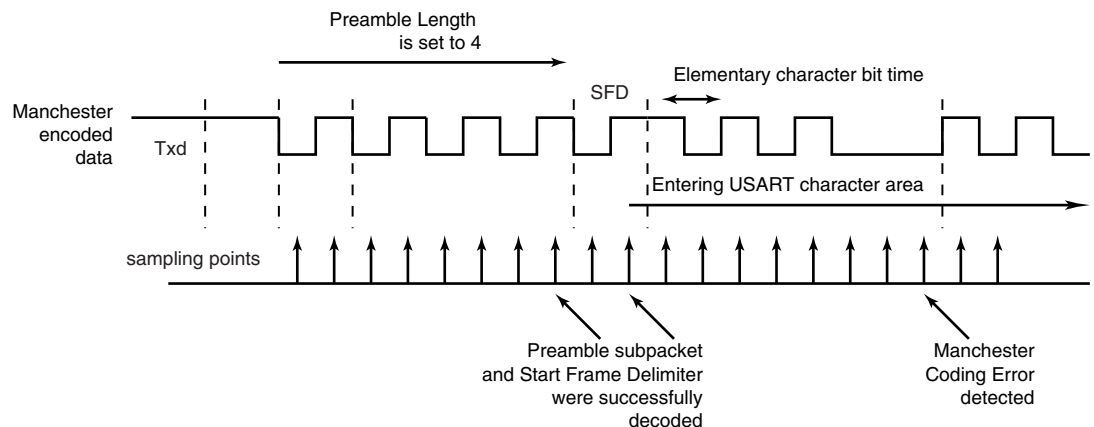
Figure 25-15. Manchester Error Flag
