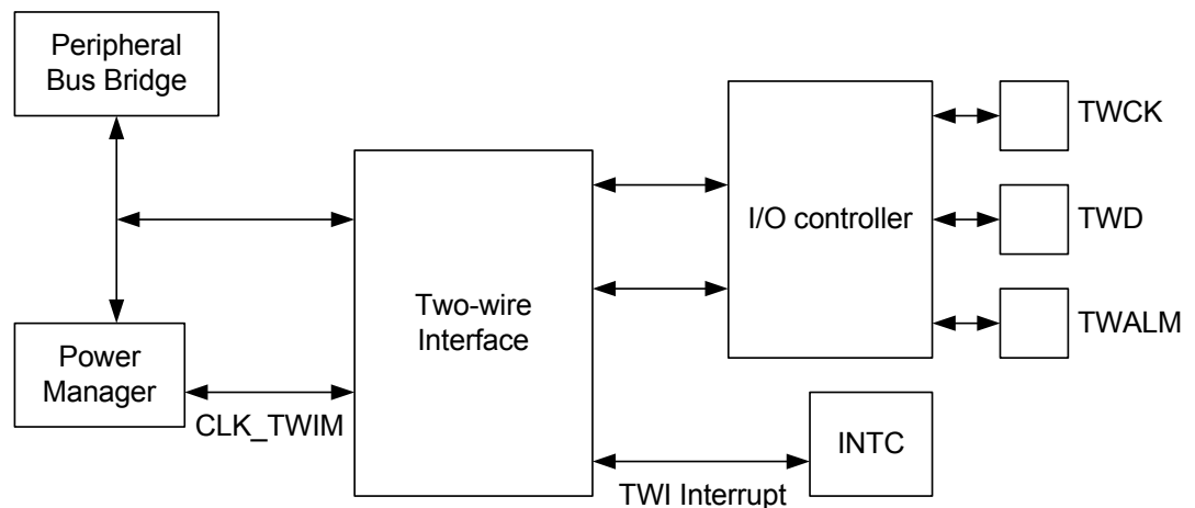
Figure 23-1. Block Diagram
