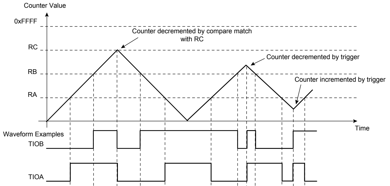
Figure 27-13. WAVSEL = 3 With Trigger
