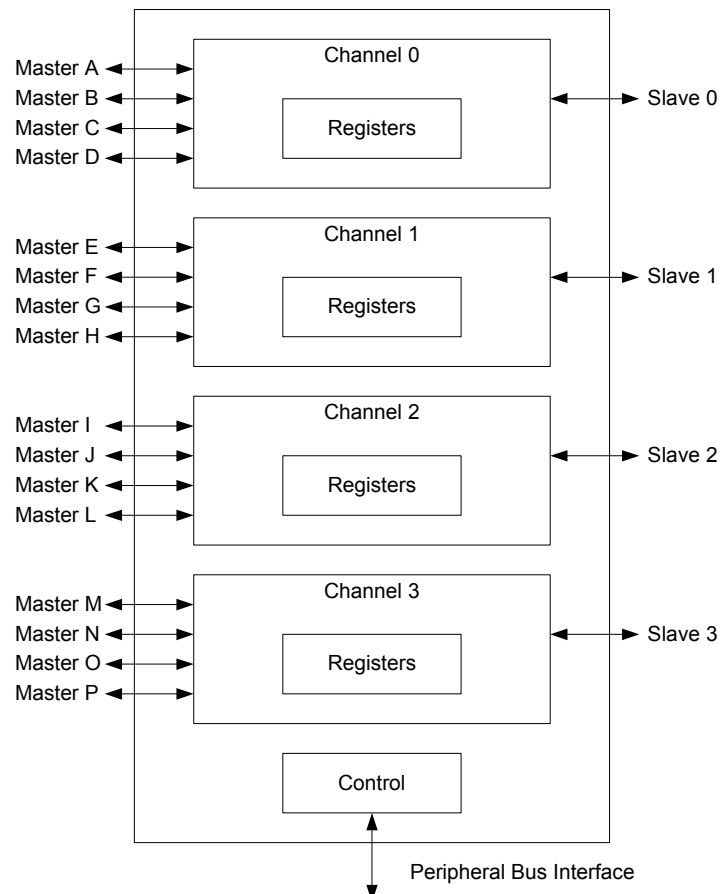
Figure 29-1. BUSMON Block Diagram
