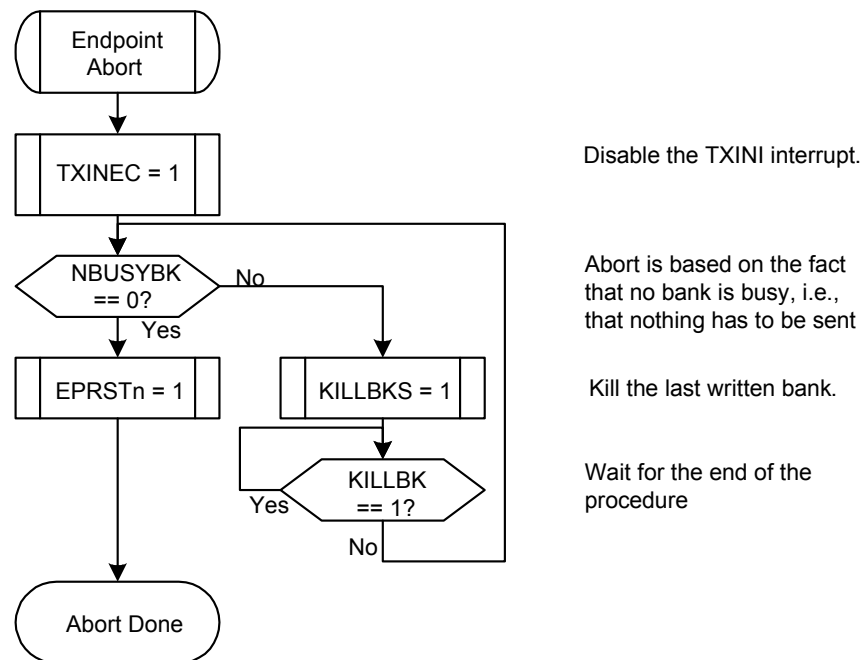
Figure 26-18. Abort Algorithm
