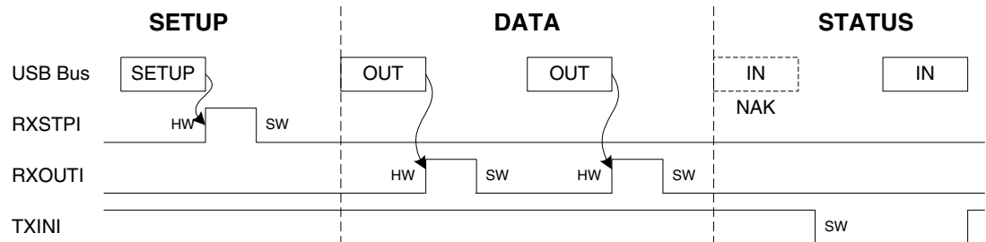
Figure 26-14. Control Write
