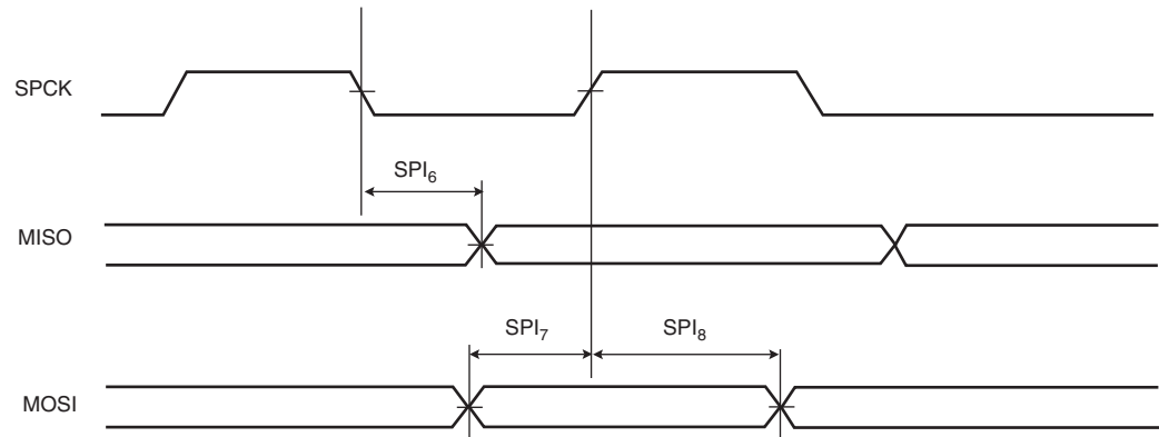
Figure 35-11. SPI Slave mode with (CPOL= 0 and NCPHA= 1) or (CPOL= 1 and NCPHA= 0)
