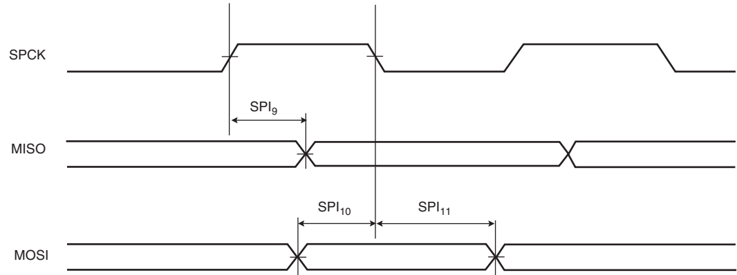
Figure 35-12. SPI Slave mode with (CPOL= NCPHA= 0) or (CPOL= NCPHA= 1)
