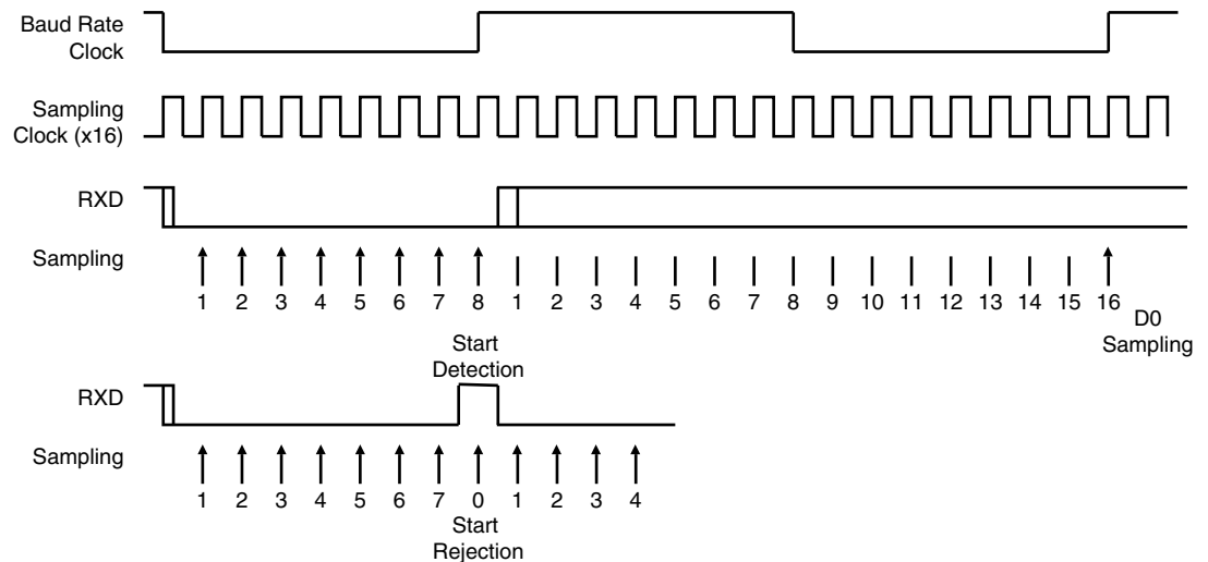
Figure 25-11. Asynchronous Start Detection
