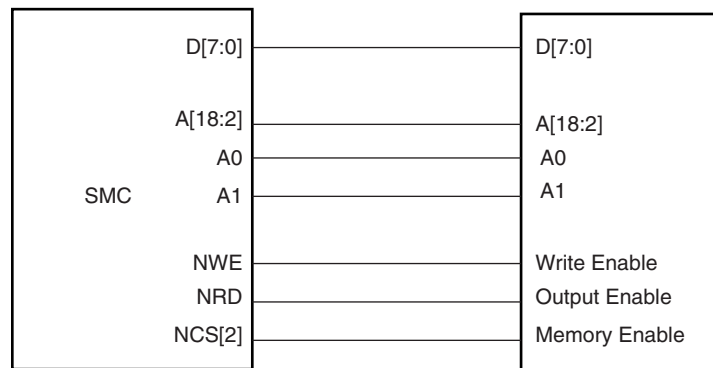
Figure 15-4. Memory Connection for an 8-bit Data Bus
