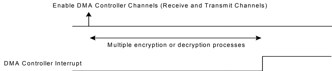
Figure 32-3. DMA Mode when MR.LOD is zero
