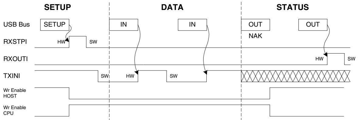
Figure 26-15. Control Read
