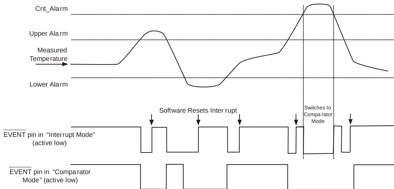
Figure 6-1. \overline{\text{EVENT}} Pin Mode Functionality
