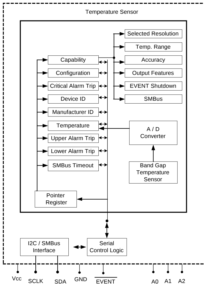
Figure 1-1. Block Diagram
