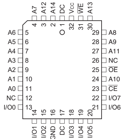
32-Pad CLCC (1)
