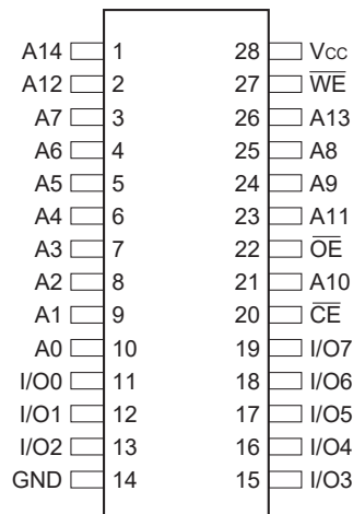
28-Lead Cerdip/Flatpack
