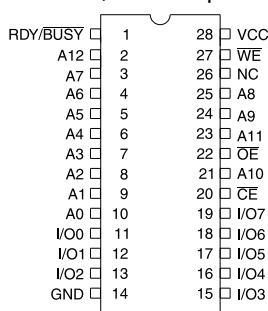
PDIP, SOIC Top View
