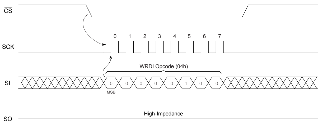
Figure 6-3. \text{WRDI} Timing
