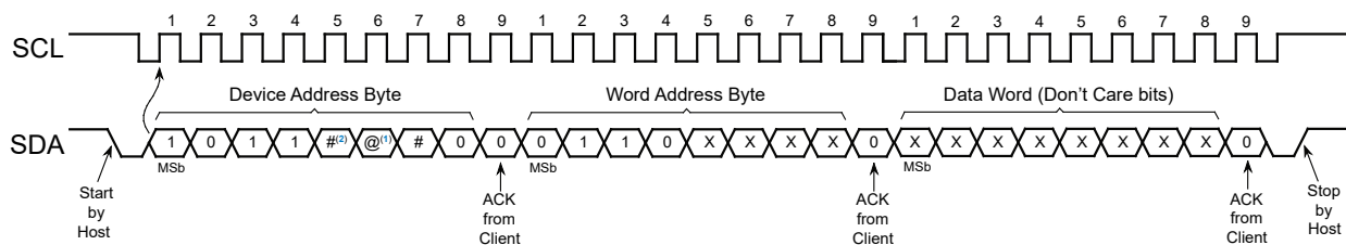
Figure 10-3. Lock Command
