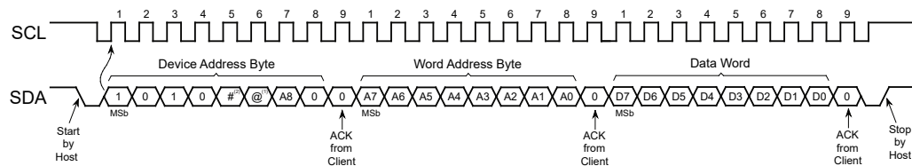
Figure 7-1. Byte Write
