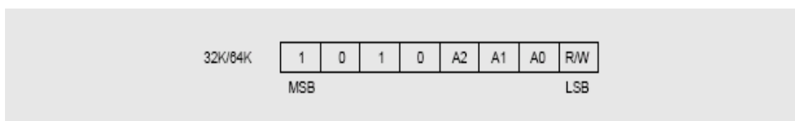
I Figure 4: Device Address
