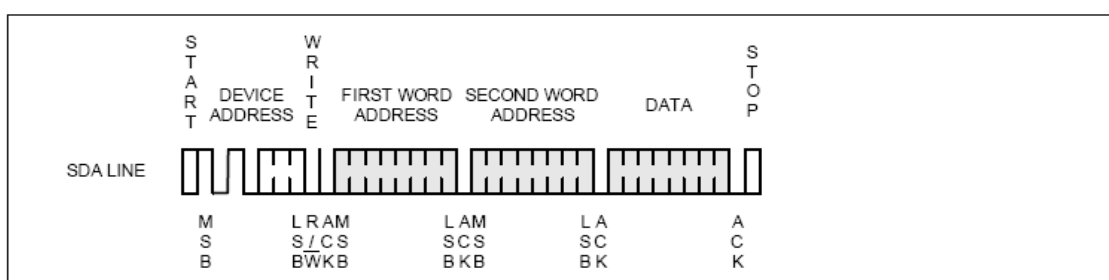
I Figure 5: Byte Write
