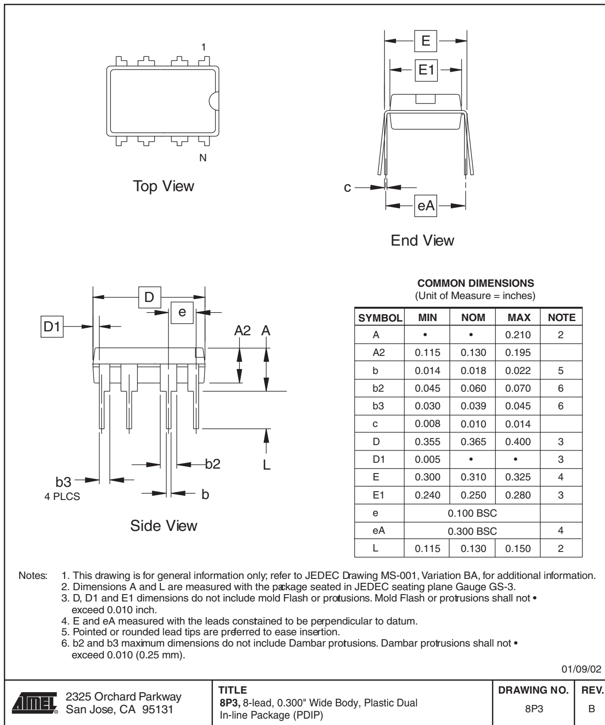
Figure 1. 8P3 – PDIP
