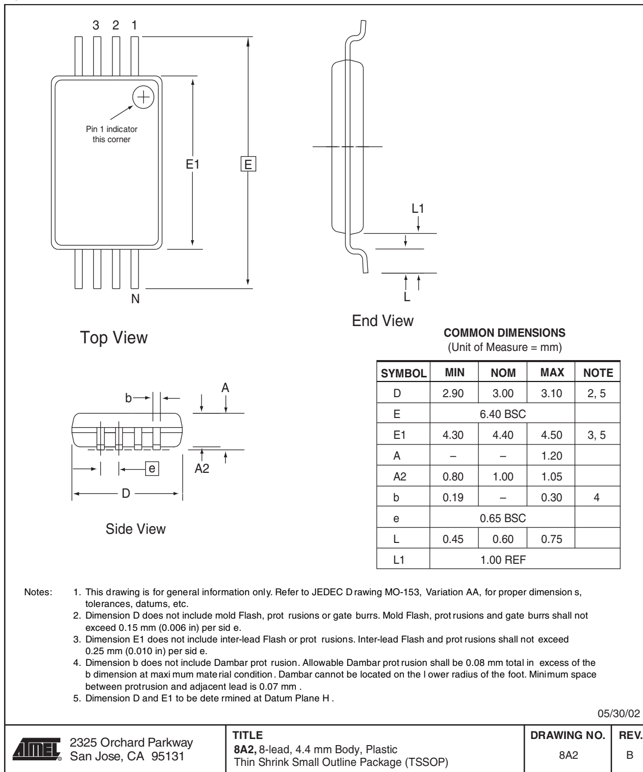
Figure 16. 8A2 – TSSOP
