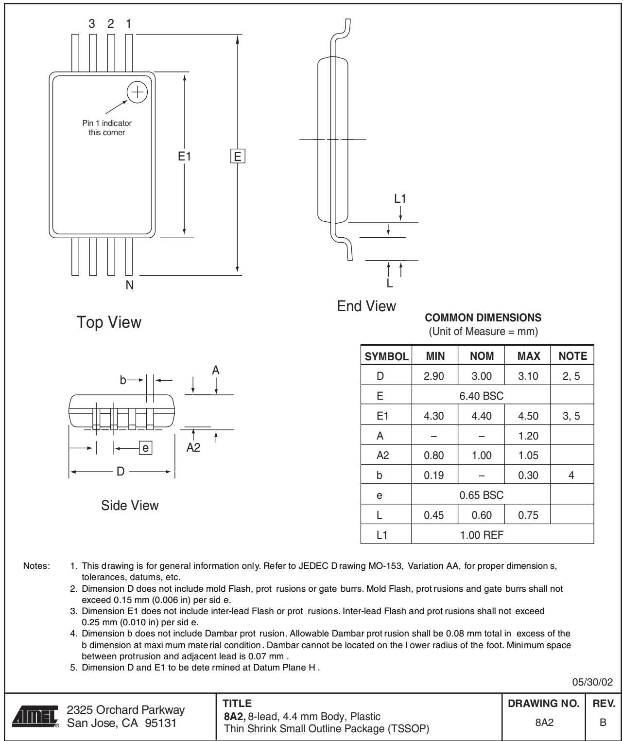
Figure 14. 8A2 – TSSOP
