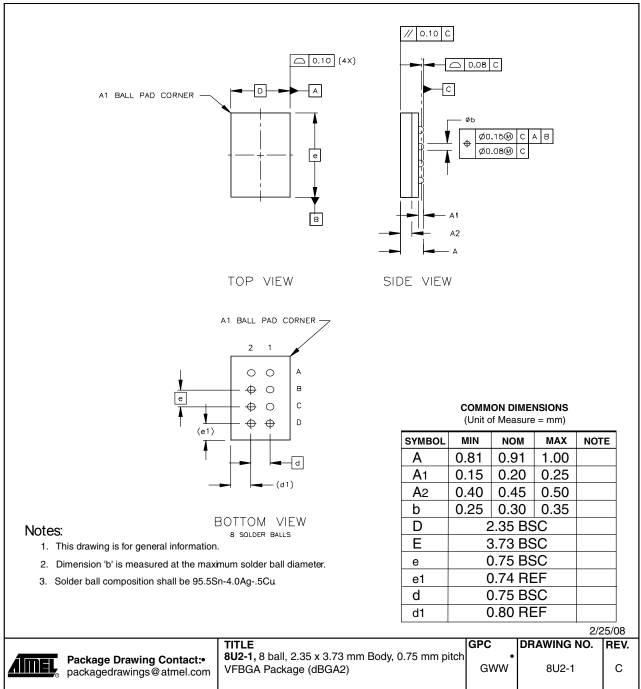
Figure 16. 8U2-1 – VFBGA
