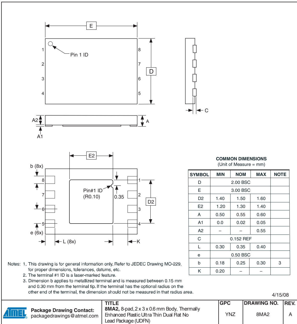
Figure 15. 8MA2 – UDFN
