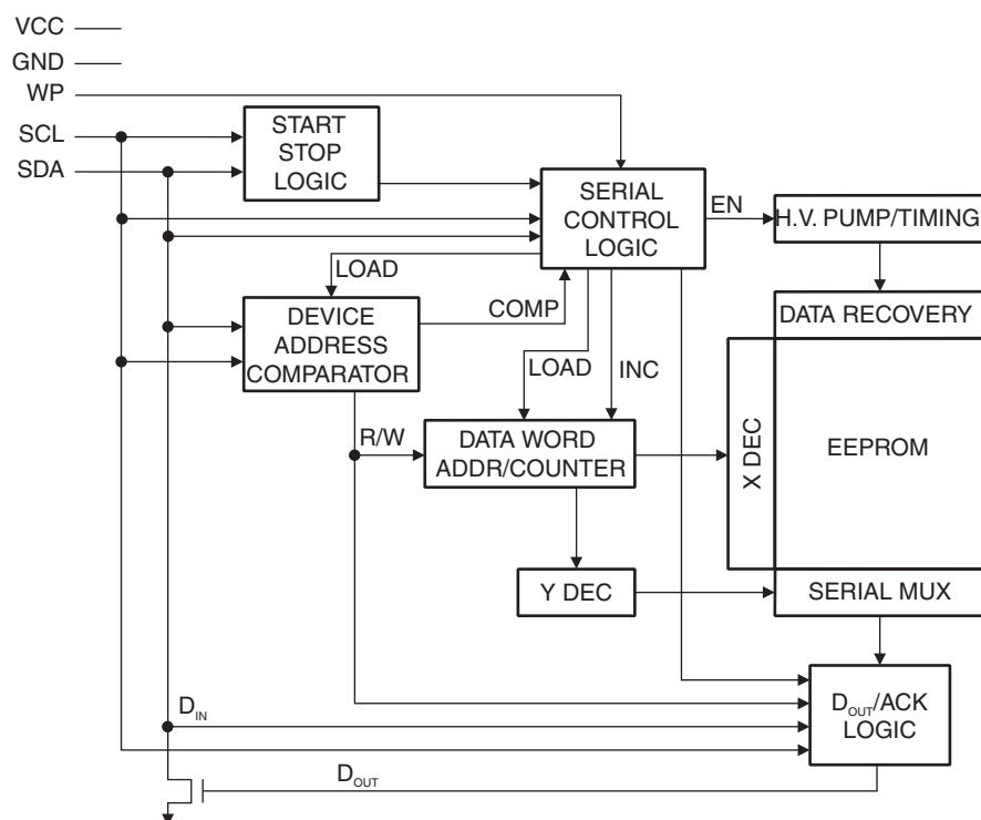
Figure 0-2. Block Diagram
