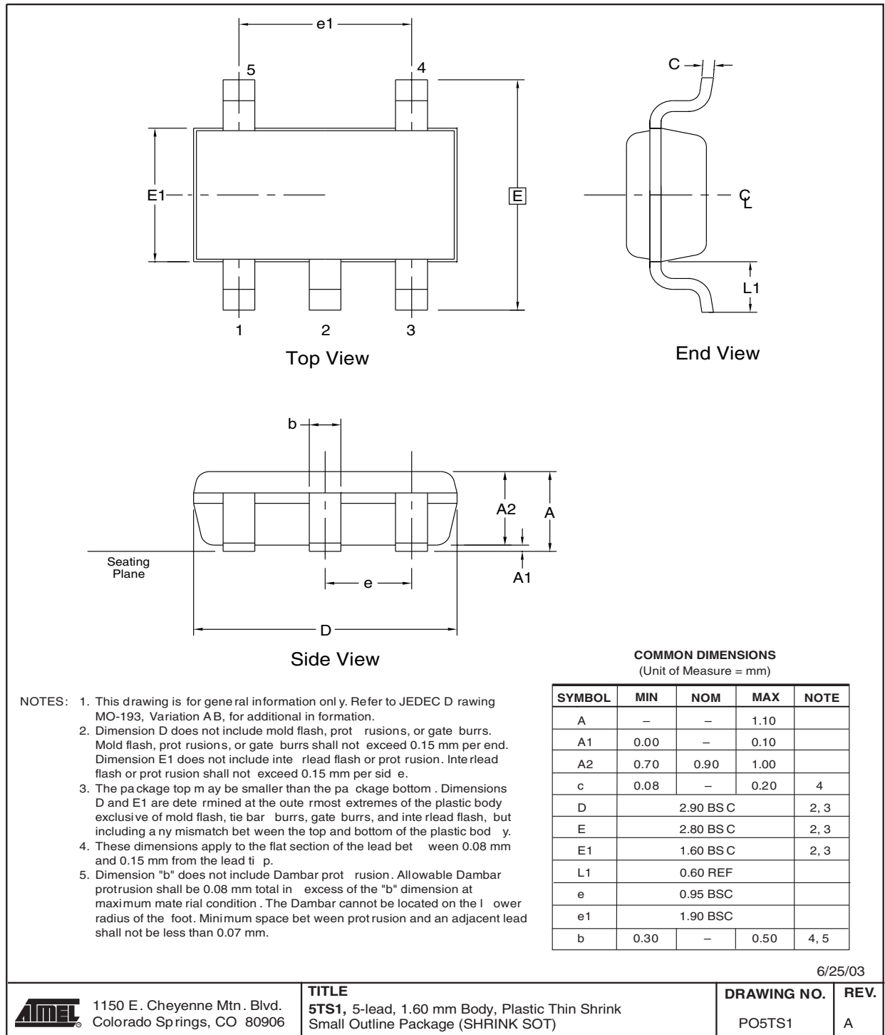
Figure 19. 5TS1 – SOT23
