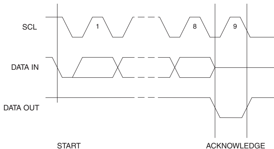
Figure 8-4. Output Acknowledge
