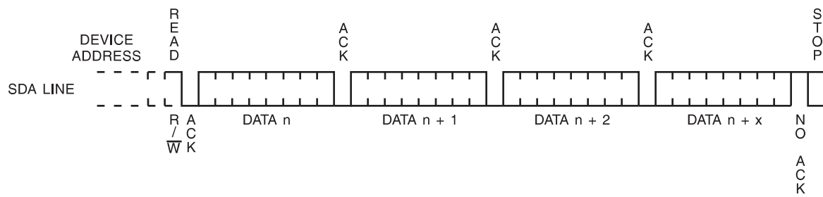
Figure 11-6. Sequential Read
