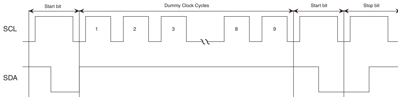
Figure 6-1. Software Reset
