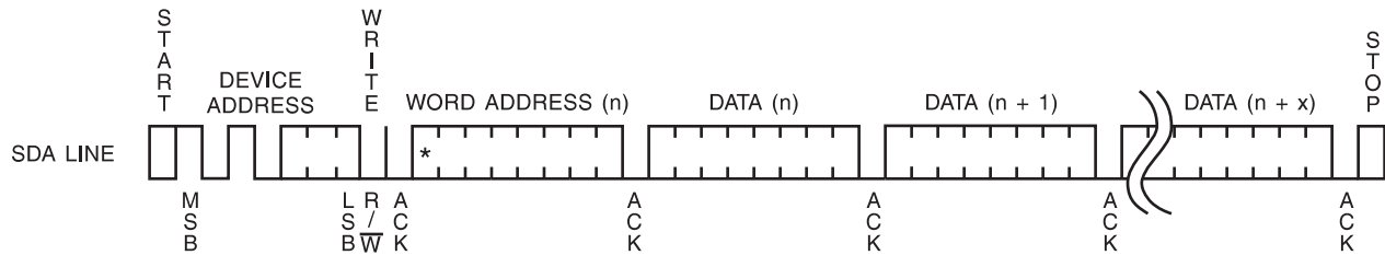
Figure 11-3. Page Write
