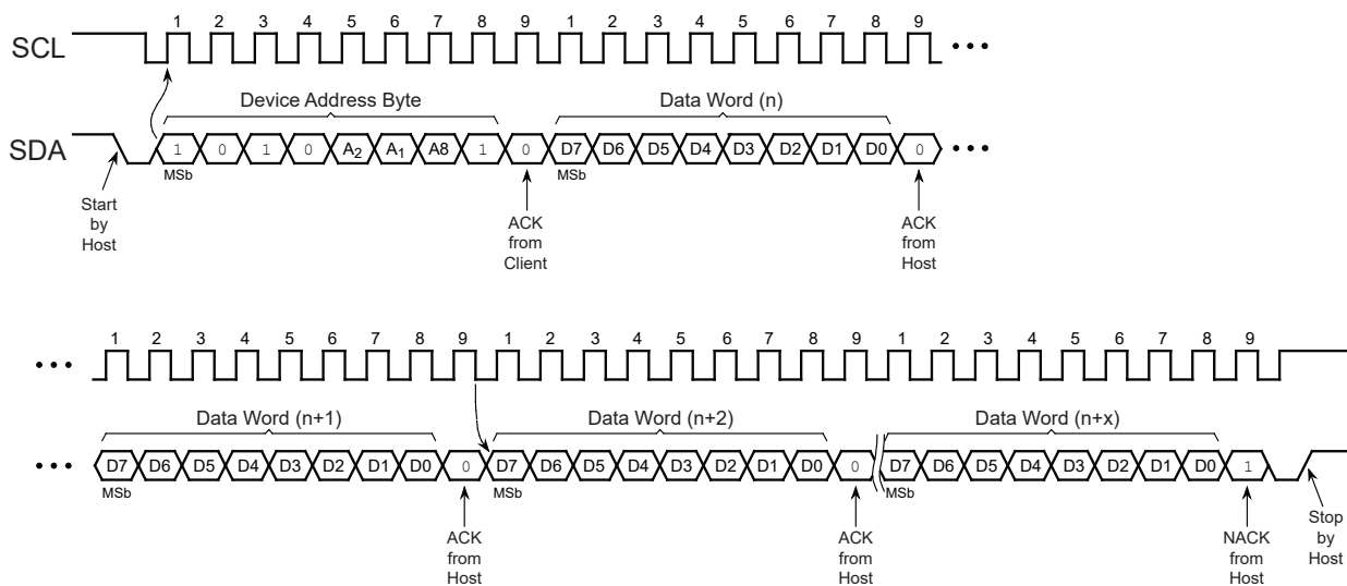
Figure 8-3. Sequential Read
