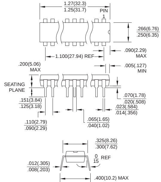
24P3 , 24-Lead, 0.300" Wide. Plastic Dual Inline Package (PDIP) Dimensions in Inches and (Millimeters) JEDEC STANDARD MS-011 AB
