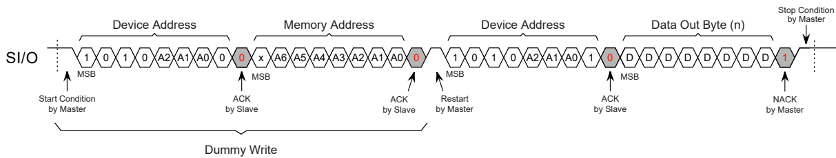
Figure 8-2. Random Read
