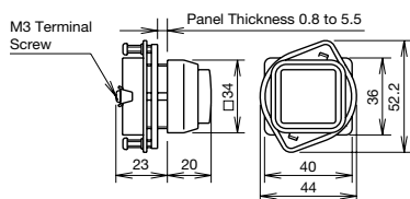
Square Full Voltage UPQN3B
