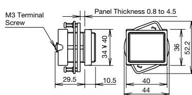
Rectangular Full Voltage UPQN4
