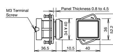
Rectangular Full Voltage UPQNE4
