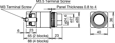
ALNE*G Momentary E16/Full Voltage
