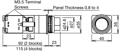
ALN*G Momentary BA9S/Transformer
