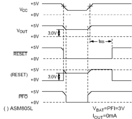
Figure 3. RESET/RESET Timing
