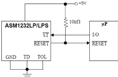
Figure 1. Typical Operating Circuit
