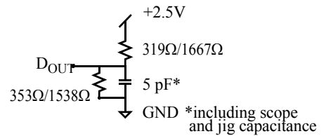
Figure C: Output load(B)
